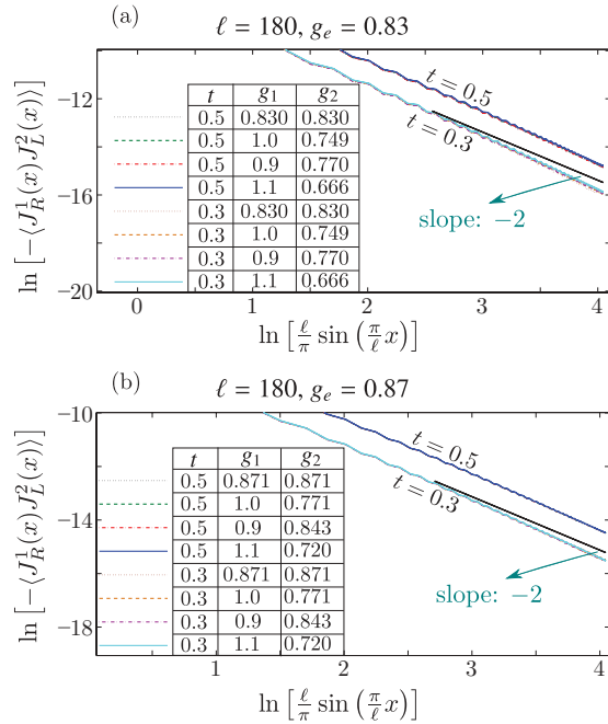
FIG. 3. (Color online) The correlation function \langle J_R^1(x)J_L^2(x) \rangle for different combinations of g_1 and g_2 corresponding to two values of g_e < 1 . The data exhibits very good collapse, and indicates a vanishing conductance.
