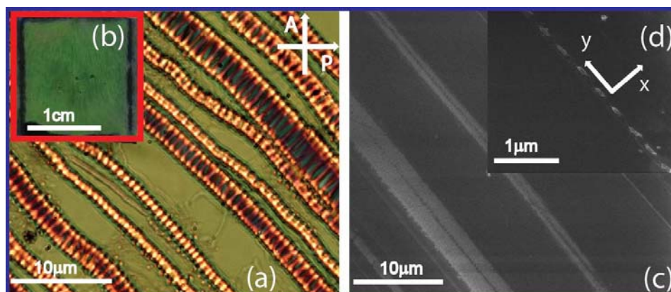
Figure 2. POM view (a) of the sample (b) along with the SEM image of morphology (c) and its high magnification (d)
