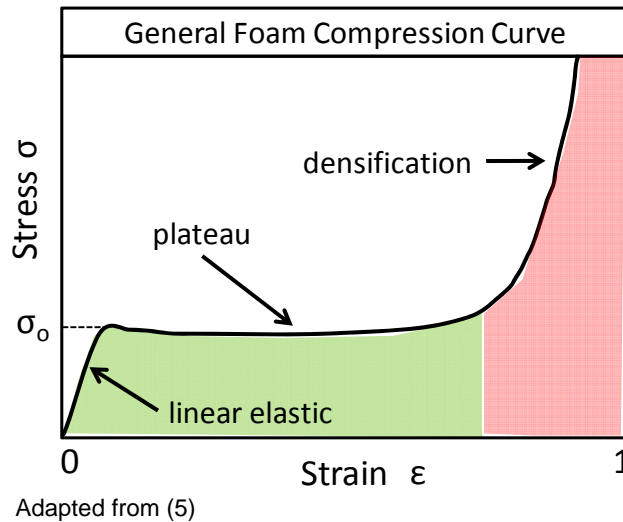
Adapted from (5) Figure 2. General stress vs. strain response of a foam material
