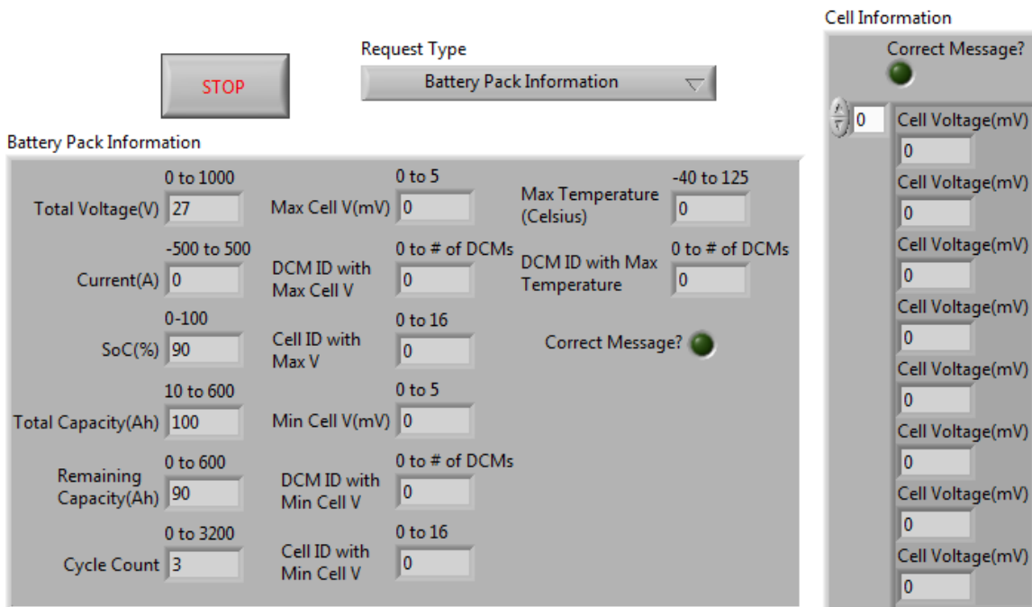
Figure 10. The Labview interface of the EMS communication VI.
