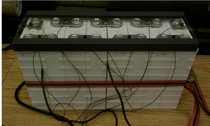
Figure 8. The assembled battery pack with wires connected to the EMS.
