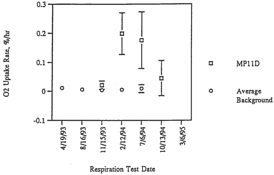
MP11D Zero Order O 2 Uptake Rates (Corrected to 12°C)
