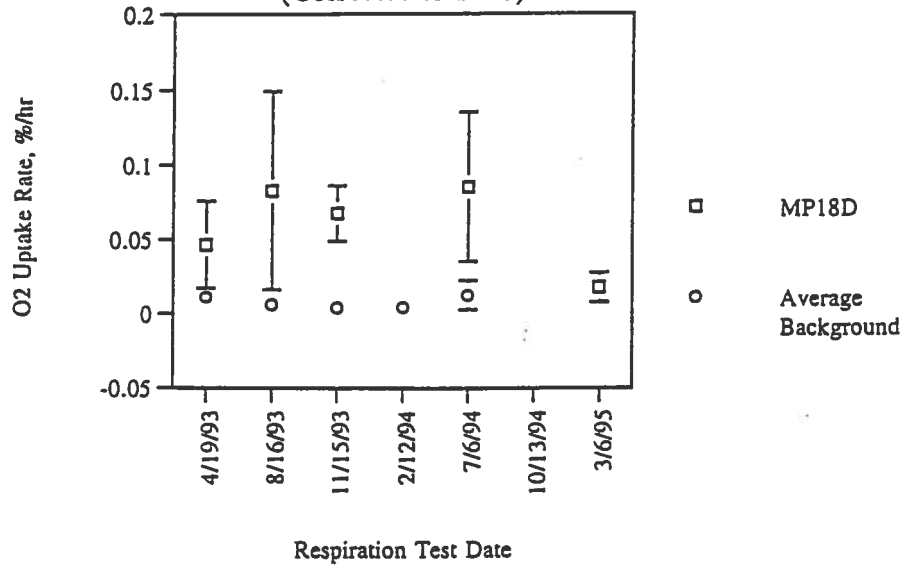
MP18D Zero Order O 2 Uptake Rates (Corrected to 12°C)
