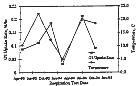
Zero Order O 2 Uptake Rate and Subsurface Temperature, MP29M
