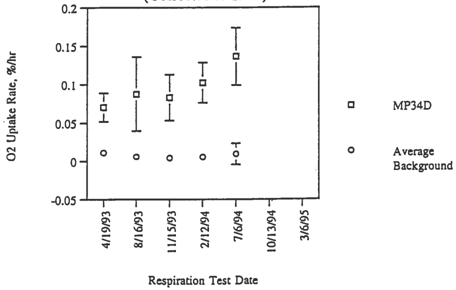
MP34D Zero Order O 2 Uptakes Rates (Corrected to 12°C)
