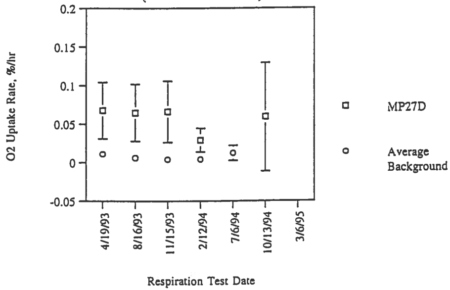
MP27D Zero Order O 2 Uptake Rates (Corrected to 12°C)
