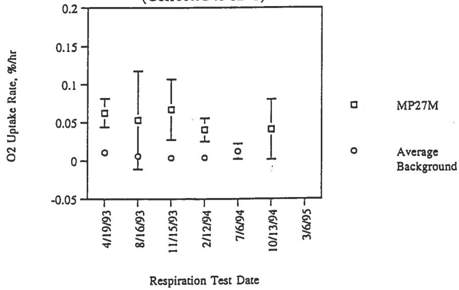
MP27M Zero Order O 2 Uptake Rates (Corrected to 12°C)
