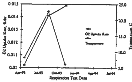
Zero Order O2 Uptake Rate and Subsurface Temperature, MP23S
