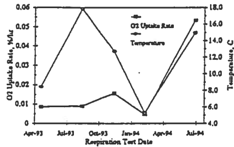
Zero Order O 2 Uptake Rate and Subsurface Temperature, MP21D
