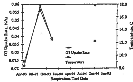
Zero Order O 2 Uptake Rate and Subsurface Temperature, MP10D
