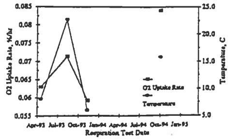
Zero Order O 2 Uptake Rate and Subsurface Temperature, MP29S
