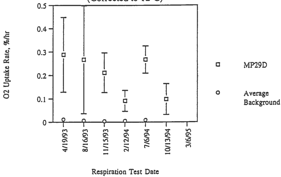
MP29D Zero Order O 2 Uptake Rates (Corrected to 12°C)
