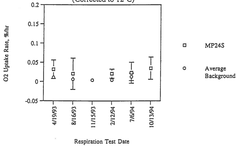
MP24S Zero Order O 2 Uptake Rates (Corrected to 12°C)
