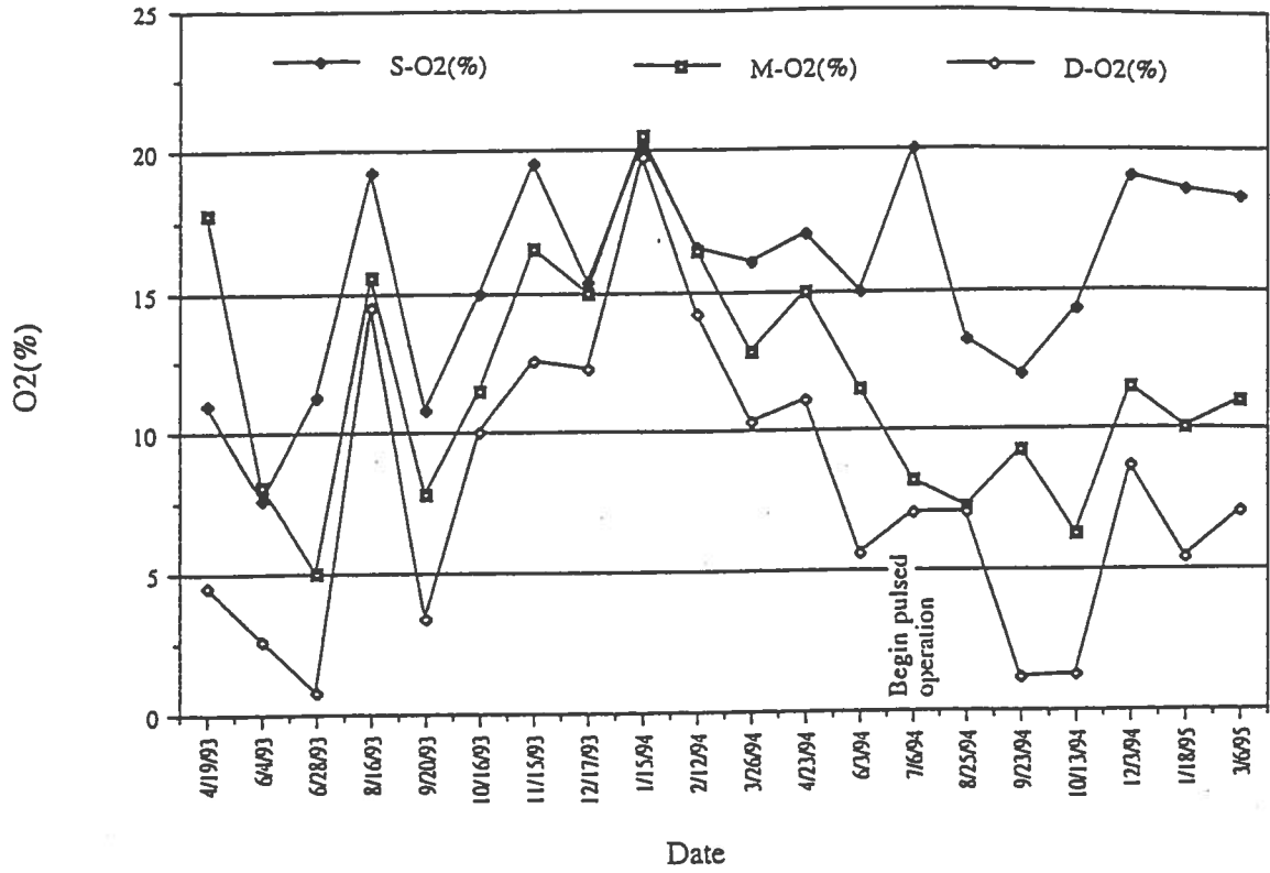
Measured O2 Concentrations at MP-5, FPTA No. 1, FE Warren AFB
