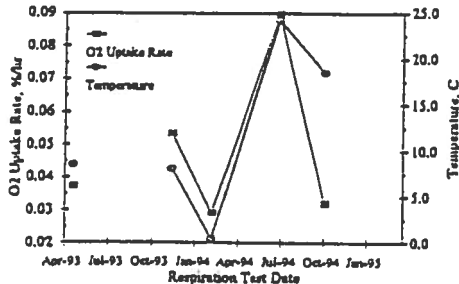
Zero Order O 2 Uptake Rate and Subsurface Temperature, MP4S
