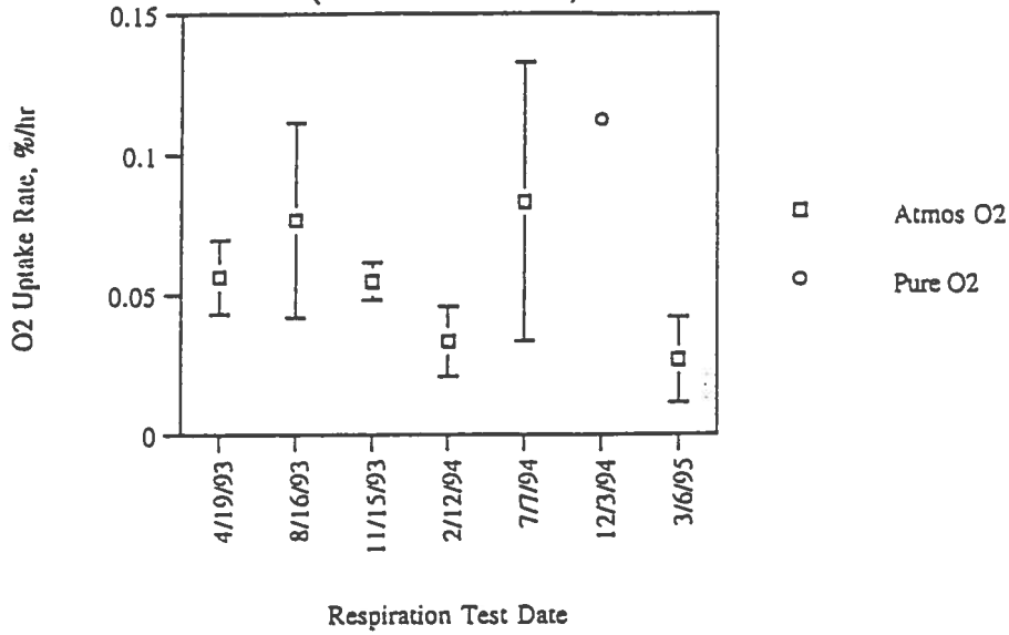
MP13D Zero Order O 2 Uptake Rates (Corrected to 12°C)
