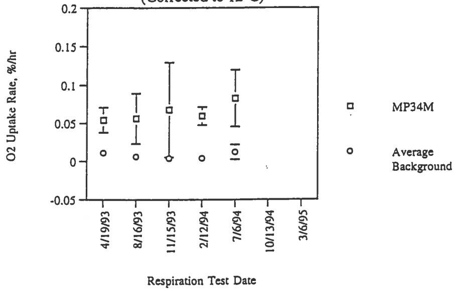
MP34M Zero Order O 2 Uptake Rates (Corrected to 12°C)
