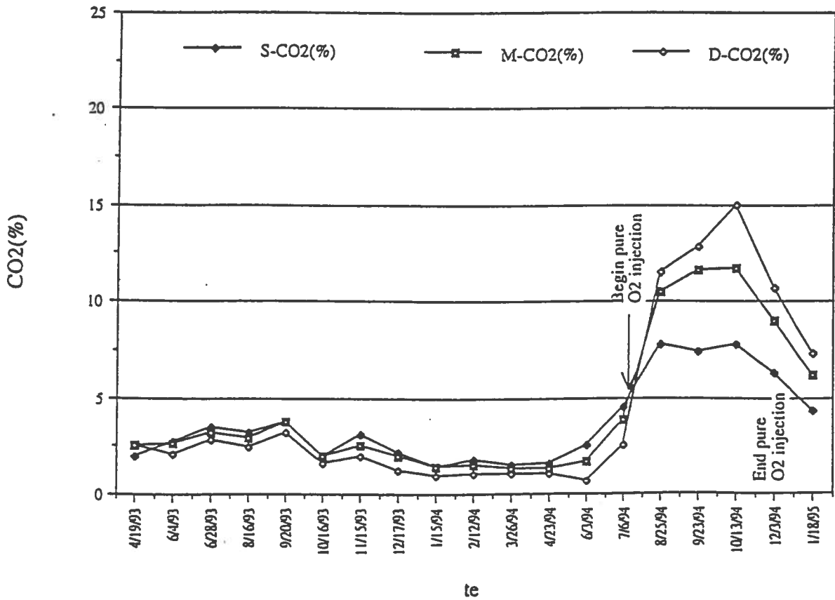
Measured CO2 Concentrations at MP-14, FPTA No. 1, FE Warren AFB
