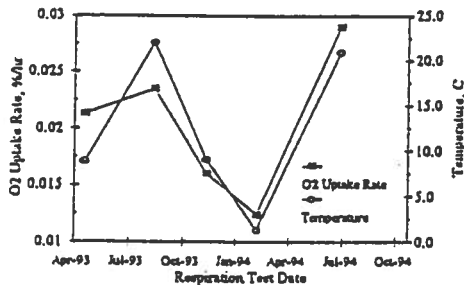
Zero Order O 2 Uptake Rate and Subsurface Temperature, MP12M
