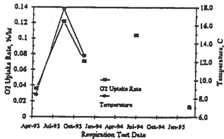
Zero Order O 2 Uptake Rate and Subsurface Temperature, MP18D
