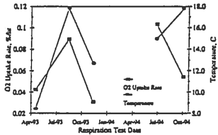
Zero Order O2 Uptake Rate and Subsurface Temperature, MP24D
