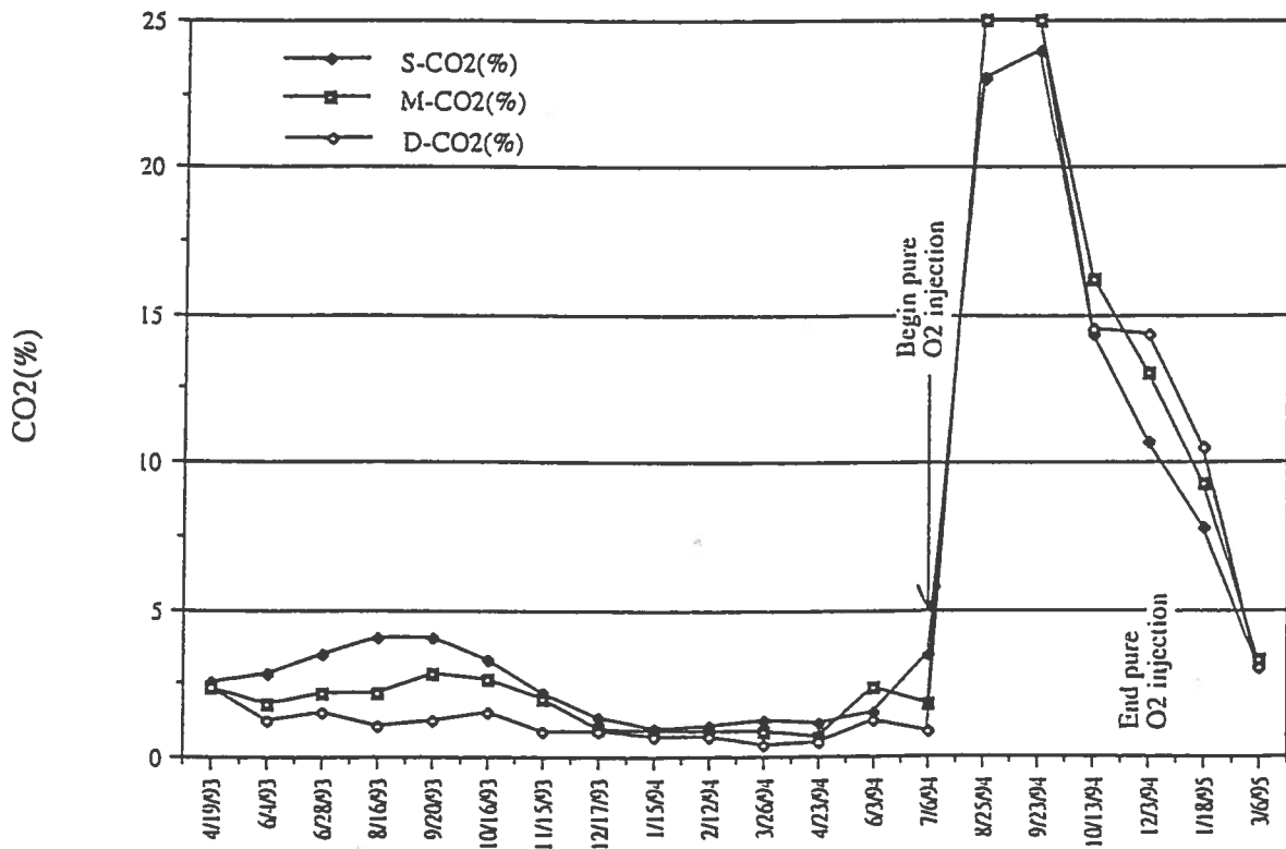
Measured CO2 Concentrations at MP-19, FPTA No. 1, FE Warren AFB
