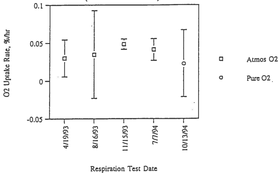
MP18M Zero Order O 2 Uptake Rates (Corrected to 12°C)
