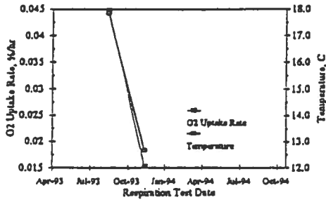
Zero Order O 2 Uptake Rate and Subsurface Temperature, MP8D
