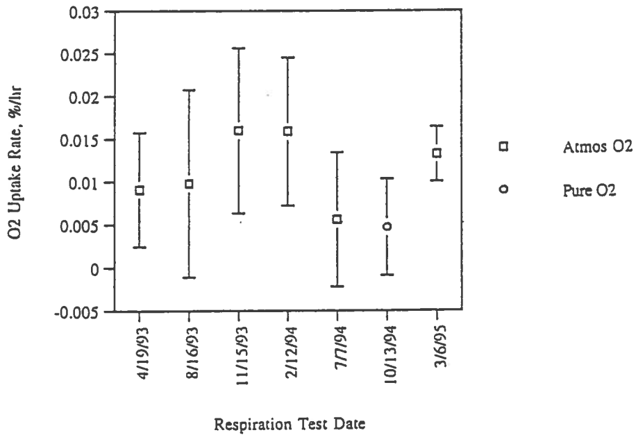
MP14S Zero Order O 2 Uptake Rates (Corrected to 12°C)
