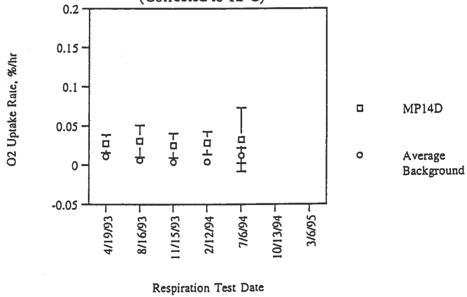
MP14D Zero Order O 2 Uptake Rates (Corrected to 12°C)
