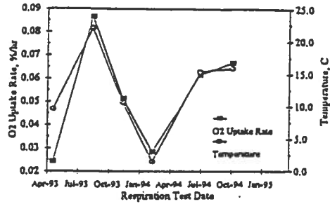
Zero Order O 2 Uptake Rate and Subsurface Temperature, MP6M
