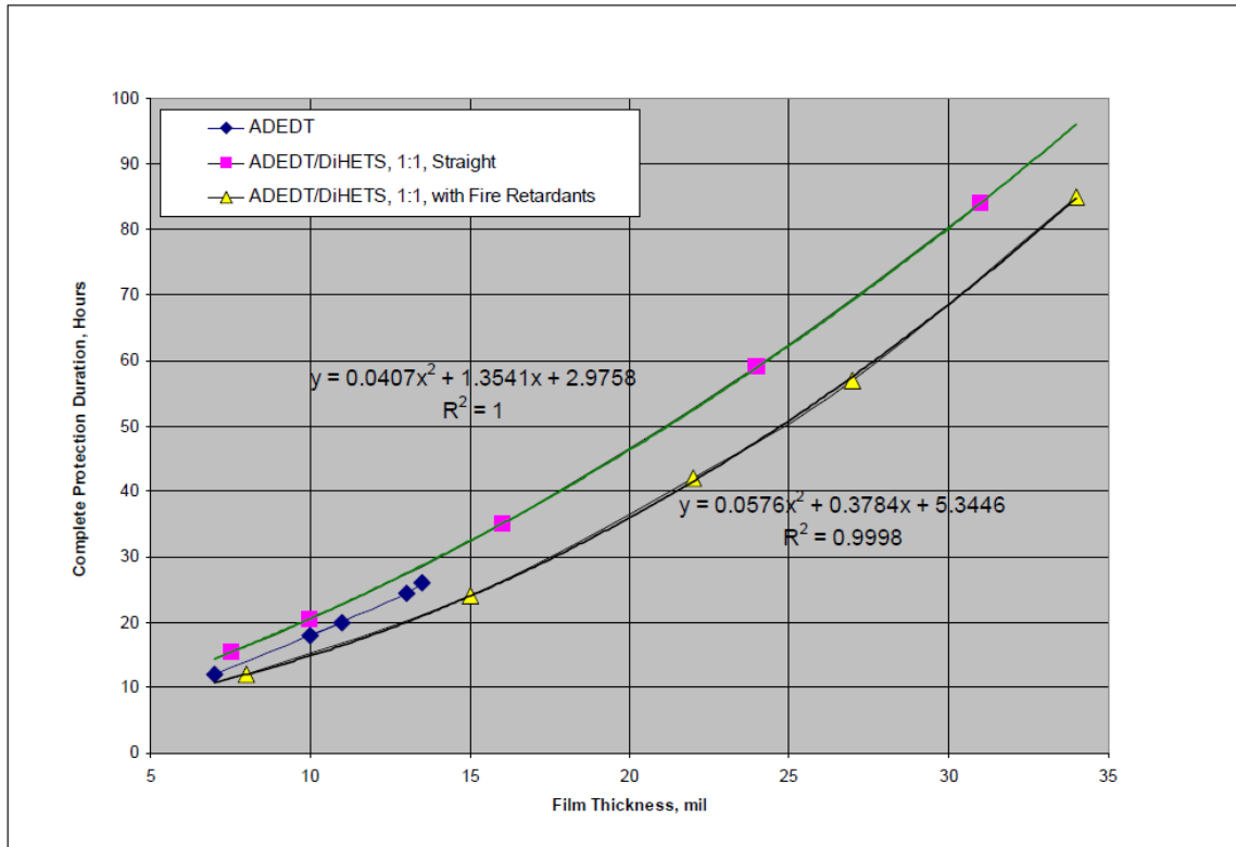
Fig. 6. Duration of protection vs. thickness of films for different formulations
