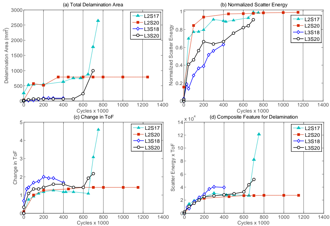
Figure 4. (a) Delamination area as observed from X-ray (b) Normalized scatter energy. (c) Time of flight and (c) Composite feature for delamination.
