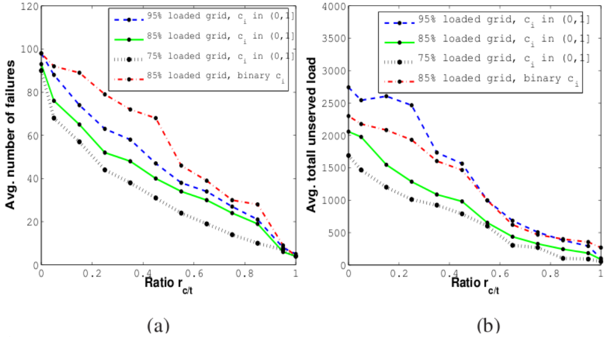
Fig. 6. Average (a) number of failed lines, and (b) total unserved load, due to cascading failures as a function of the ratio of total controllable loads over the total load in the grid.
