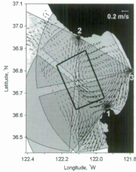
Figure 8. Setting of the gap simulation experiments: Gray shading shows data acquisition areas of the radars in the presence of a simulated ship (case b ) moving across the Monterey Bay. Area within the rectangle shows the boundary of the data-free region in case c . Numbers enumerate radars switched off in case d .
