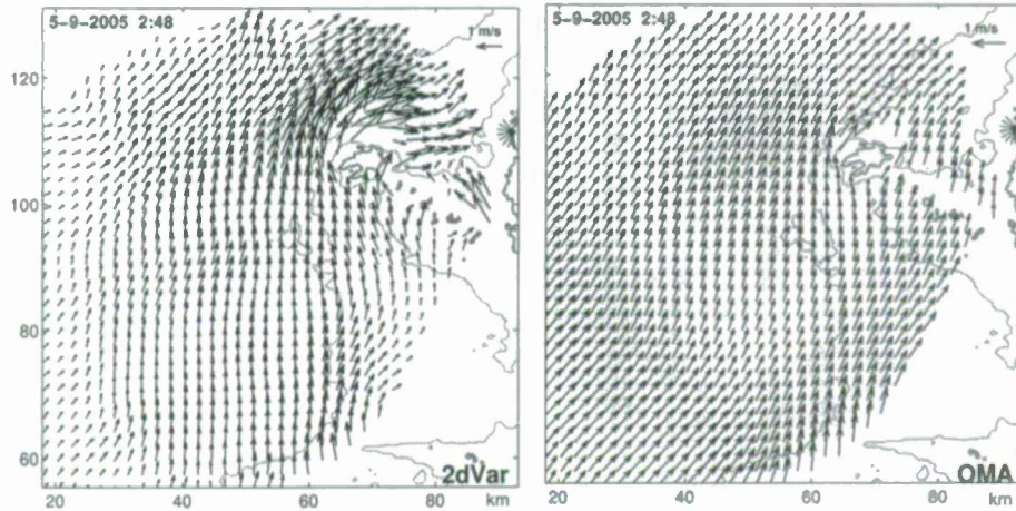
Figure 7. Surface currents in the Iroise Sea (Northern Bay of Biscay) on September 5, 2005 (02:48 GMT) obtained by the 2dVar (left) and OMA methods. 50 and 100m isobaths are shown by gray contours. HFR location at Point Garchine is shown by the black dot.
