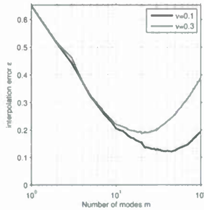
Figure 9. Interpolation error \epsilon as a function of the number of modes m .
