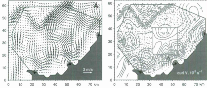
Figure 1. Setting of the numerical experiments: Left panel shows the "true" velocity field \mathbf{u}' which has nine eddy structures superimposed on two jets: one following the coastline and another located farther offshore. The right panel shows the vorticity field \text{curl} \mathbf{u}' . Three coastal radars sample the radial velocities along beam directions binned at 2 km radial and 5^\circ azimuthal resolution. Sampling points are shown by gray dots. Gray rectangle in the upper right panel envelops simulated gap in the HFR data. Radar positions are shown by black dots on the coastline. The interpolation domain and the coastline are similar to the ones used in [20] for OMA processing of HFR observations in the Bodega Bay. The coordinate system is rotated clockwise (north is on the right). Contour interval for vorticity is 5 \cdot 10^{-5} \text{ s}^{-1} .
