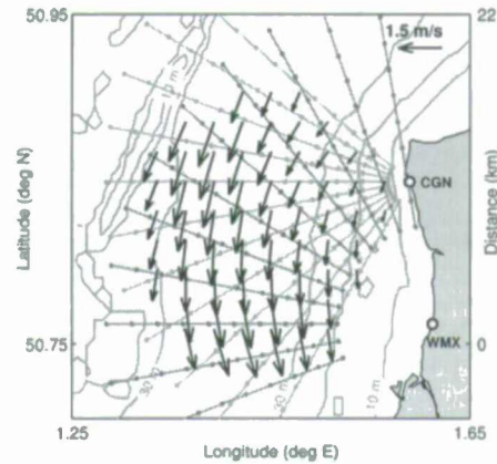
Figure 12. Surface velocity at 14.20 GMT on May 21 2003 in the ERMANO study area. Contours show the bathymetry in meters. Gray dots indicate locations of the surface velocity measurements by two radars (shown by circles).
