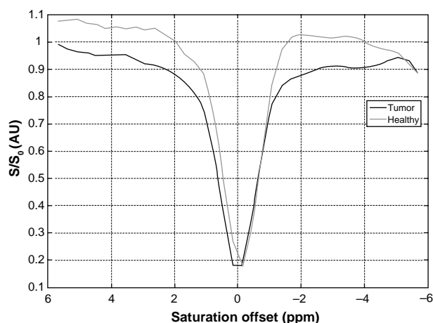
Figure 6 Example z-spectra arising from a CEST MRI experiment at 3 T. Note: The normalized signal ( S/S_0 ) is shown as a function of saturation offset frequency for regions of interest in malignant tumor (black line) and healthy fibroglandular tissue (gray line).
