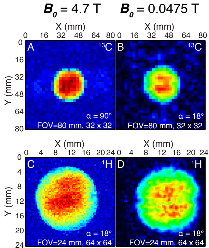
Figure 11. 13 C and 1 H MRI of sodium 1- 13 C-acetate. 4.7 T acquisition used Boltzmann 13 C P = 4.06 \cdot 10^{-6} and 1 H P = 1.61 \cdot 10^{-5} , and 0.0475 T used approximately the same polarization levels, 13 C P = 4.70 \cdot 10^{-6} and 1 H P = 1.05 \cdot 10^{-5} . All measurements used a spherical phantom: for 1 H 1.0 g sodium 1- 13 C-acetate in 99.8% D 2 O with 2.8 mL total volume and for 13 C 5.18 g sodium 1- 13 C-acetate in 99.8% D 2 O with 17.5 mL total volume. All acquisition and processing parameters were identical except 13 C excitation pulse angle \alpha . No image extrapolation or zero filling was used.
