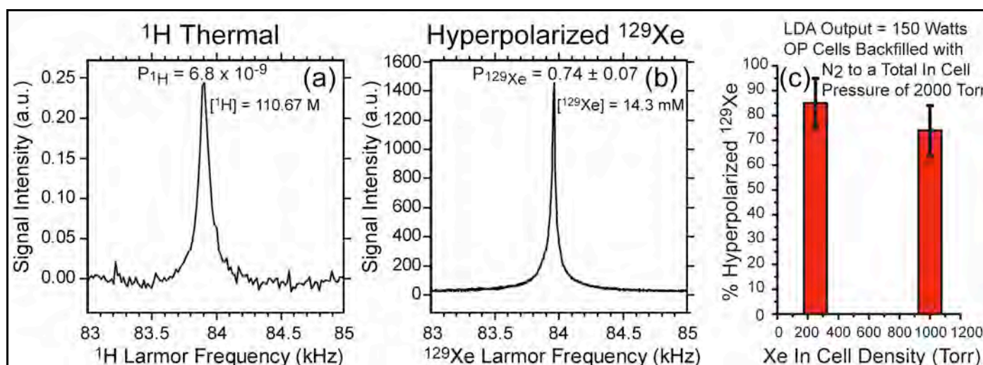
Figure 8. In situ NMR spectroscopy at 84 kHz. (a) 1 H reference (Thermal) spectrum obtained from water, [ 1 H] = 110.7 M, doped with 10 mM CuSO 4 inside 0.50 L OP cell. Spectrum was acquired at 84 kHz 1 H Larmor frequency, with 100,000 averages using 1 H thermal polarization P = 6.8 \times 10^{-9} . (b) 129 Xe spectrum (nat. ab. = 26.44%) of 1000 torr Xe, [ 129 Xe] = 14.3 mM, backfilled with N 2 to a total cell pressure of 2000 torr acquired at 84 kHz 129 Xe Larmor frequency with 1 scan. Both spectra were taken using the same circuit-detection coil with the same B_1 tipping angle. (c) Bar graph representing % P_{Xe} at 250 and 1000 torr with ~85% and 74% xenon polarization respectively.
