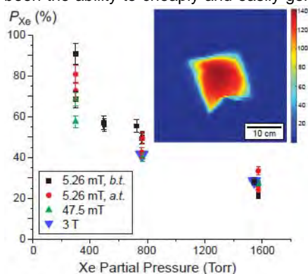
Fig. 1 (left): P_{\text{Xe}} values measured at 5.26 mT, 47.5 mT, and/or 3 T, plotted versus xenon partial pressure during SEOP. Labels ‘b.t.’ and ‘a.t.’ respectively refer to measurement obtained “before” and “after” Xe gas was transferred to another container. Inset: 2D FLASH ^{129}\text{Xe} projection image of HPXe in a Tedlar bag following transport to 3 T (FOV: 40 cm; slice thickness: 1.7 cm; TE/TR: 2.6/5.1 ms, flip angle: -4^\circ ; SNR \sim 40:1 ).
