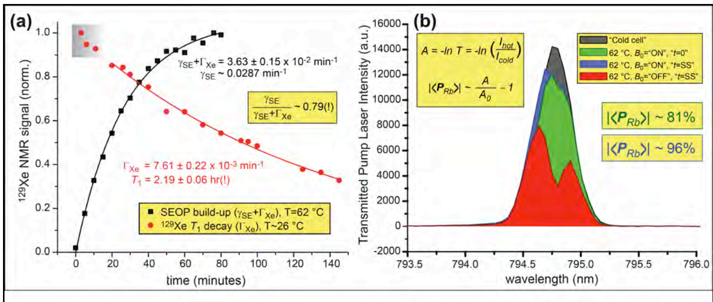
Figure 9. (a) Time-dependent in situ ^{129}\text{Xe} low-field NMR for 1000 Torr Xe, 1000 Torr \text{N}_2 . The black curve is P_{\text{Xe}} build-up during SEOP at 62\text{ }^\circ\text{C} ; the red curve is subsequent ^{129}\text{Xe} decay after the laser was turned off and the cell was cooled. Both datasets were fit to simple exponentials (curves); red data points were obtained with rf pulses possessing half the tipping angle. Red data points obtained before the cell reached room temperature (grey highlight) were not included in the fit. Losses from rf pulses were ignored during the fits. (b) In situ monitoring of global Rb electron spin polarization. Examples of near-IR spectra of the pump laser transmitted through the cell acquired under the following conditions: 1000 Torr Xe, 1000 Torr \text{N}_2 ; room temperature ("cold cell"); 62\text{ }^\circ\text{C} and B_0 = 7.13\text{ mT} at the beginning of SEOP (" t=0 "); 62\text{ }^\circ\text{C} and B_0 = 7.13\text{ mT} at steady-state for P_{\text{Xe}} (" t = \text{SS} ", see adjacent figure); and 62\text{ }^\circ\text{C} and B_0 = 0\text{ mT} at steady-state. The large changes in transmitted laser intensity when the field is cycled indicate high Rb electronic spin polarization (see inset).
