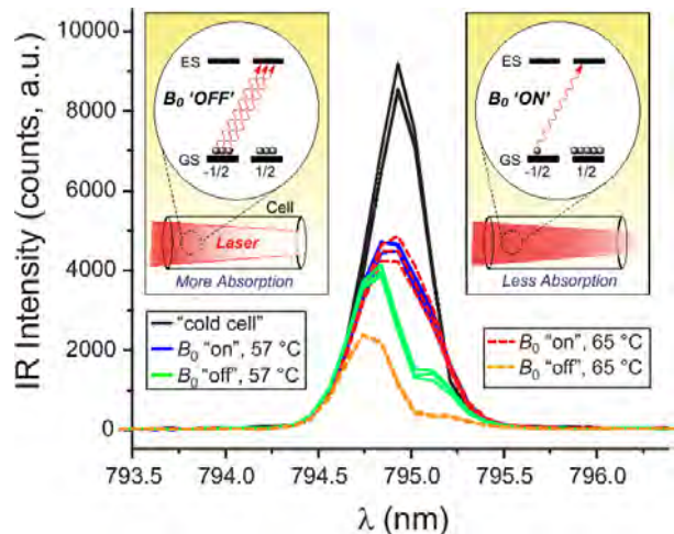
Fig. 2. (color online) In situ monitoring of global Rb electron spin polarization. Main figure: Examples of near-IR spectra of the pump laser transmitted through the cell acquired under the following conditions: room temperature ("cold cell", black solid lines); 57 °C and B_0=5.26 mT (blue solid lines); 57 °C and B_0=0 mT (green solid lines); 65 °C and B_0=5.26 mT (red dashed lines); and 65 °C and B_0=0 mT (orange dashed lines). Three scans for each condition are shown; error bars for \langle P_{Rb} \rangle values were determined by propagating the standard deviations of spectral integral values. Insets: Cartoons showing the effects of depletion pumping of electronic spin states of the alkali metal vapor on the transmitted laser intensity (assuming OP with with \sigma^+ circularly polarized light; nuclear spin levels are not shown for simplicity). When the external magnetic field B_0 is 'off' (left), optical pumping is highly inefficient, resulting in near-equal populations of the ground electronic spin states ( m_j=+1/2 & -1/2 ) and a relatively high density of absorbers in the gas phase. The presence of an applied magnetic field provides a quantization axis and results in more efficient optical pumping. This results in unequal ground state populations, corresponding to high electronic spin polarization; the reduced number of atoms in the m_j=-1/2 ground state gives rise to increased laser transmission (right).
