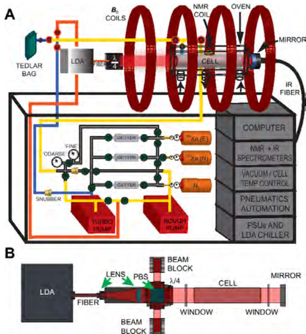
Fig. 1. (color online) The XeNA polarizer. (A) Schematic of the polarizer's key components (the liquid N 2 dewar that provides gas for oven heating and cooling is not shown). The optical path comprising beam expanding optics, polarizing beam-splitter cube, quarter-wave plate, and heat sinks is represented by ("M4"). For the gas cylinders, "N" and "E" designate xenon with naturally-abundant 129 Xe and isotopically-enriched 129 Xe, respectively. (B) Schematic showing the principal elements of the optical path.
