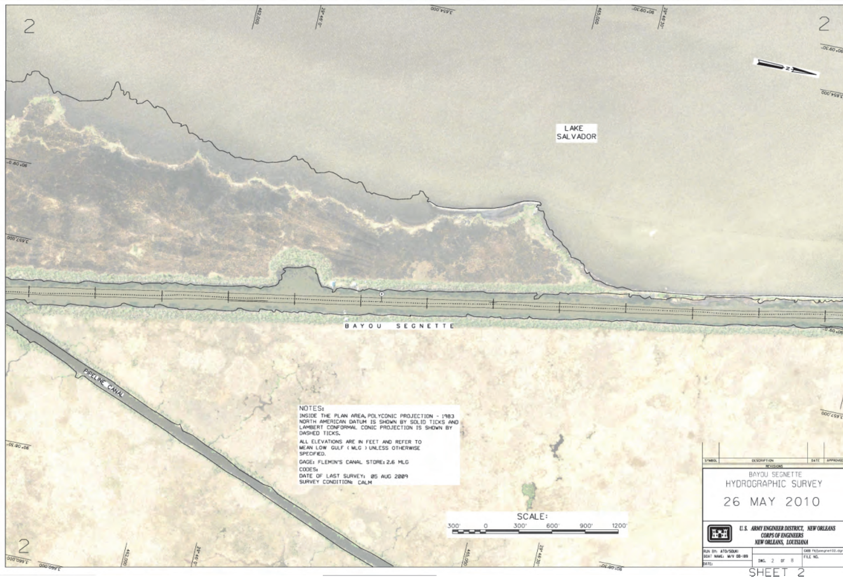
Figure A2. Bayou Segnette Waterway hydrographic survey sheet 2.
