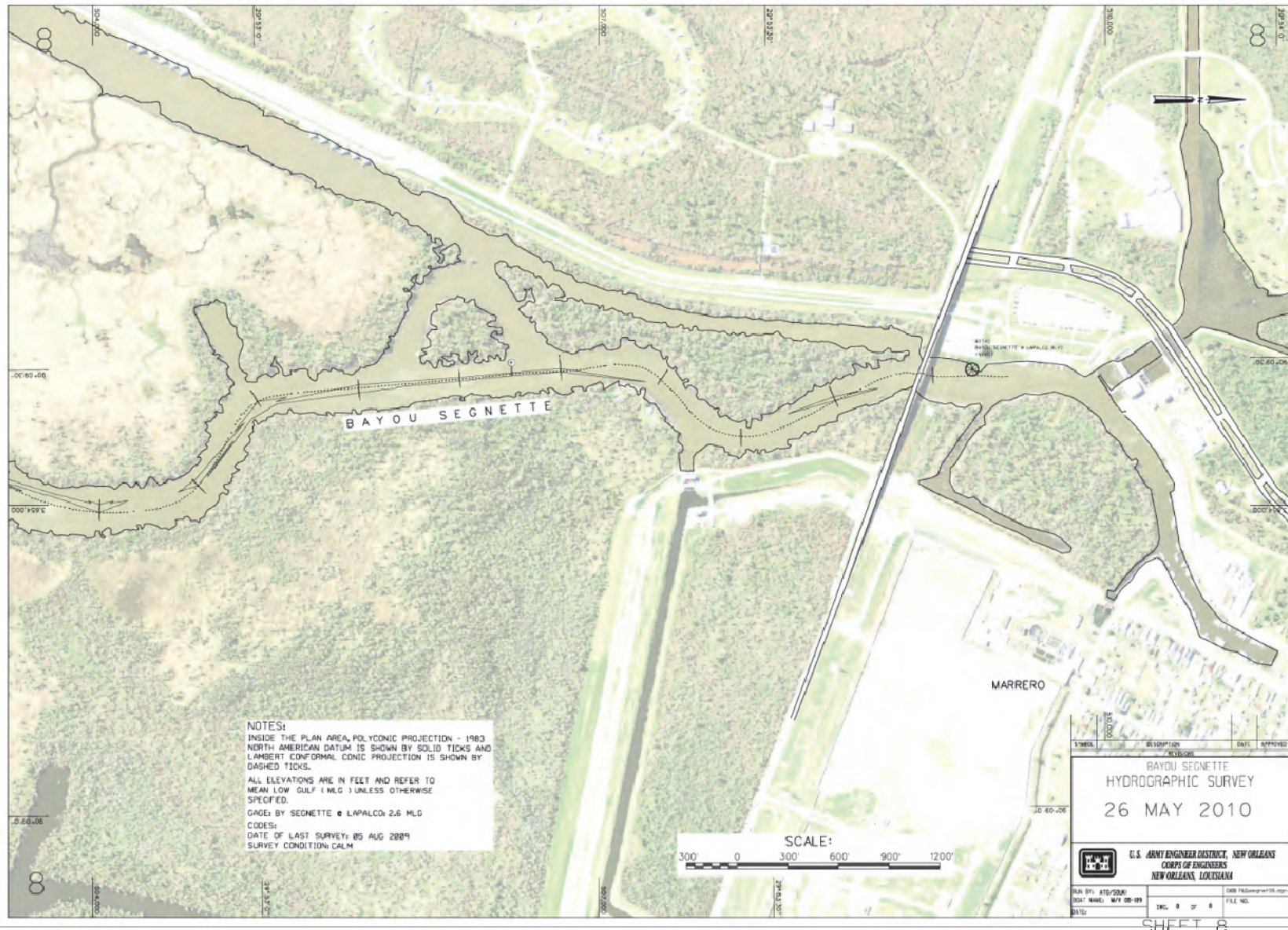
Figure A8. Bayou Segnette Waterway hydrographic survey sheet 8.
