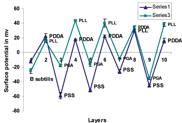
Figure 1. \zeta -potential of a B. subtilis spore in DI water at pH 6.8, showing alternation with successive deposition of cationic and anionic polyelectrolytes (synthetic: poly(dimethylallyl ammonium chloride), PDDA; sodium poly(styrene sulfonate), PSS; poly(lysine), PLL; and poly(glutamic acid), PGA).
