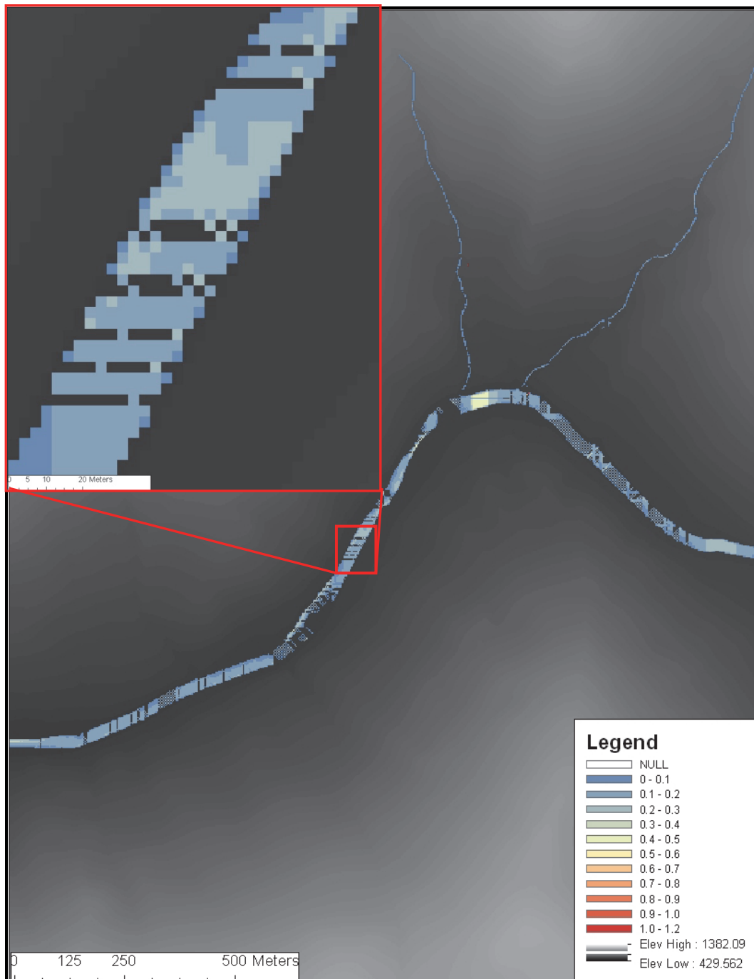
Figure 4. Example Flow Depth Output from AutoRoute
