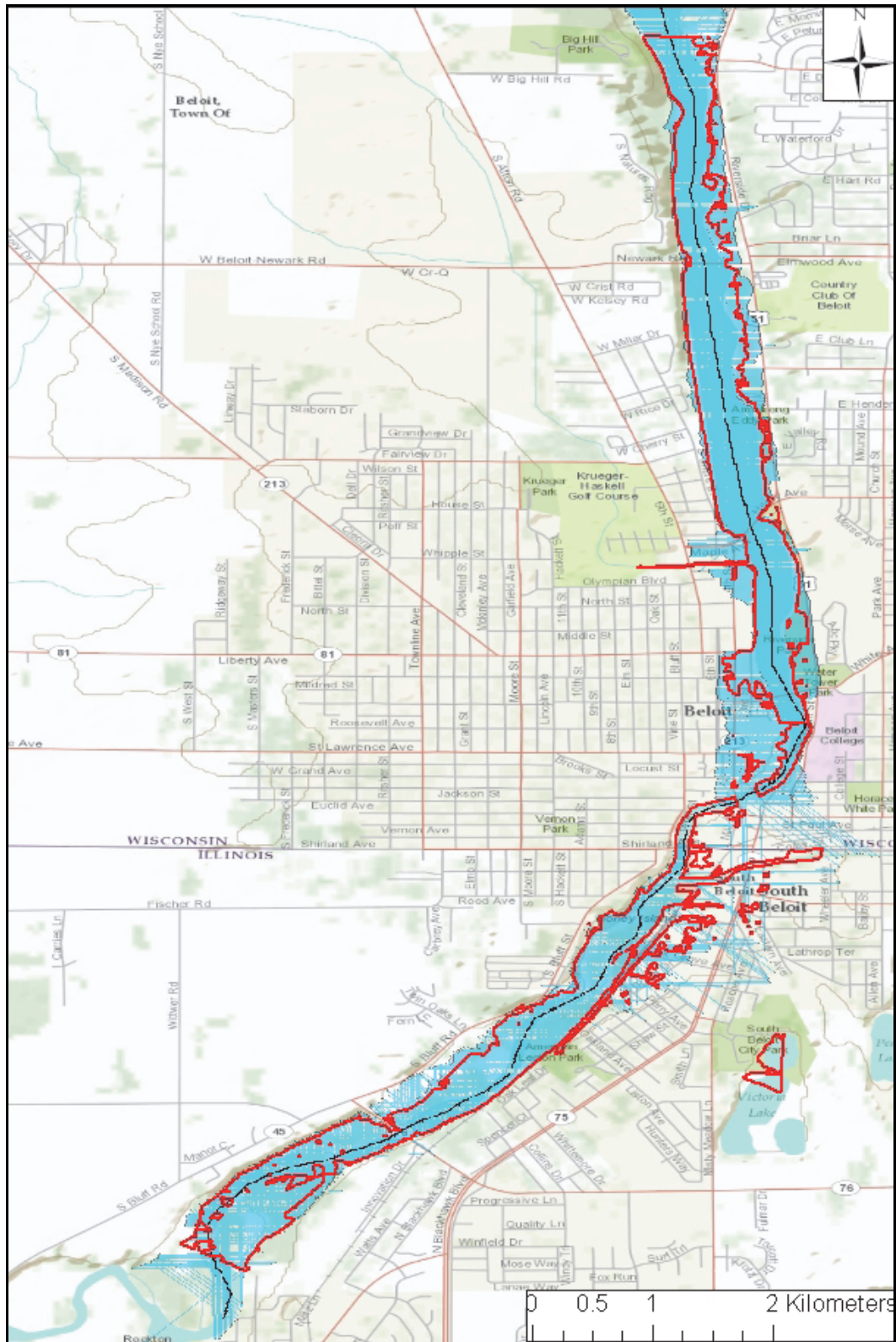
Figure 8. June 2008 Flood of Beloit, WI/IL, 10-m DEM, peak flow = 368 m 3 /s
