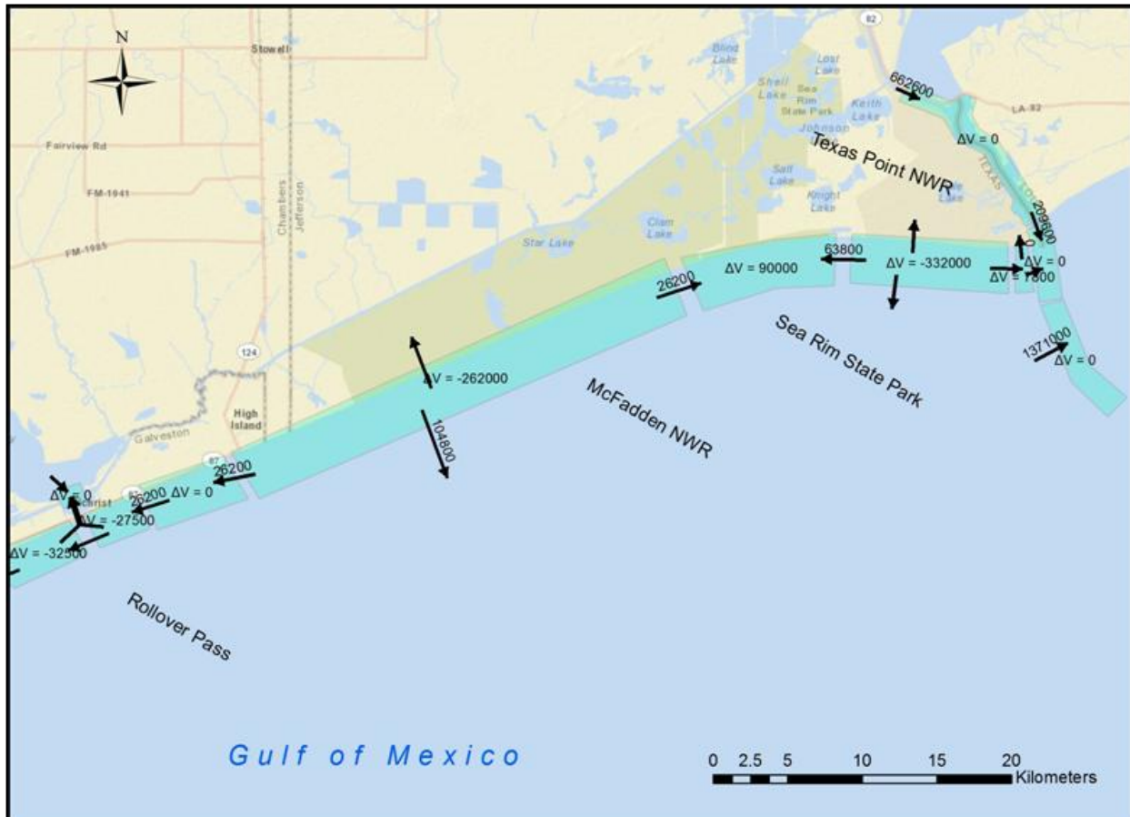
Figure 2. Sediment budget from Sabine Pass to Rollover Pass, TX (volumes in m^3/year ).
