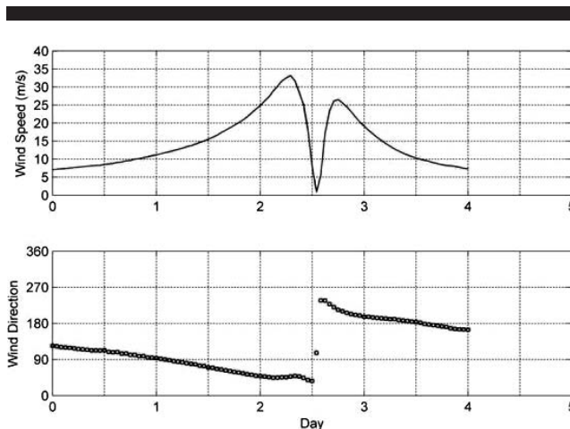
Figure 6. Wind speed and direction of the 100-year return storm.
