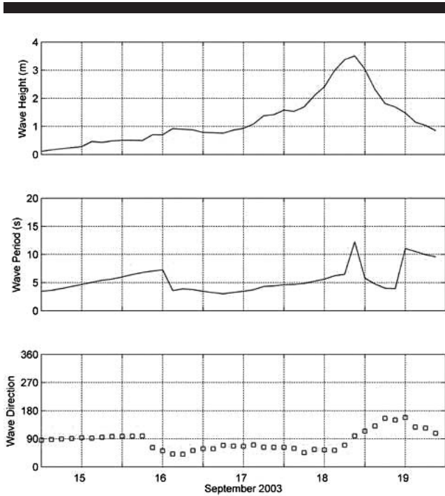
Figure 11. Wave parameters of Hurricane Isabel.
