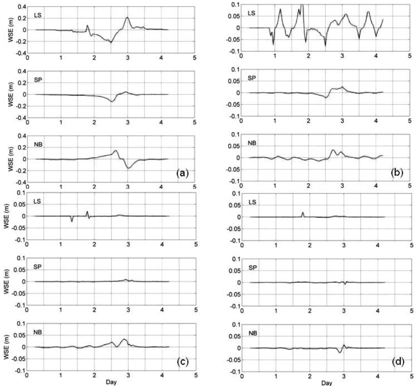
Figure 19. Water-surface elevation differences between the final model simulation and (a) the simulation without the wind forcing, (b) with a constant Manning n of 0.05 on land, (c) without the CMS-Wave, and (d) with the half-plane wave model under the 2-m SLR scenario for the 100-year storm at sites LS, SP, and NB.
