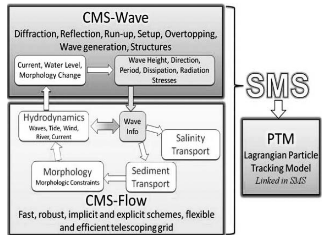
Figure 1. The CMS operational flow chart.
