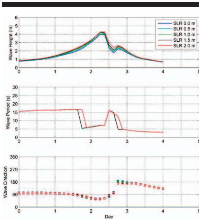
Figure 7. Wave parameters of the 100-year return storm under the existing condition and four sea-level-rise scenarios. (Color for this figure is available in the online version of this paper.)
