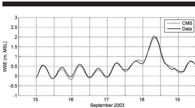
Figure 12. Water-surface elevation comparison between the calculations and measurements of Hurricane Isabel at Sewells Point, Virginia.
