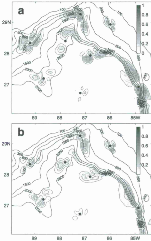
FIG. 5. Absolute difference between eight columns of the true correlation matrix for the Gaussian model (Fig. 3a) and its DL approximations (a) C_i^e and (b) C_i^r obtained with 50 ensemble members. Filled circles show locations of the diagonal elements.
