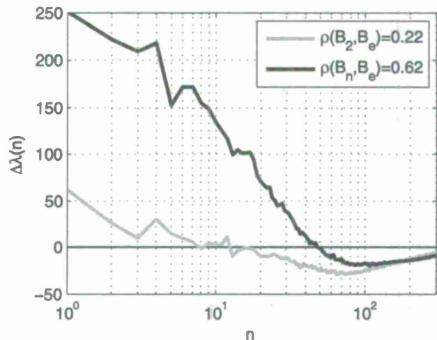
FIG. 7. Difference between the 300 largest eigenvalues of B_2 and B_e (gray line) and of B_n and B_e (top right). Distances between the corresponding matrices are shown.
