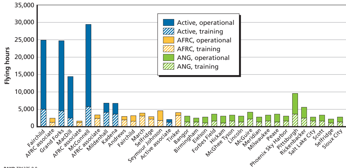
Figure B.9 Average Annual Flying Hours, KC-135 Wings
