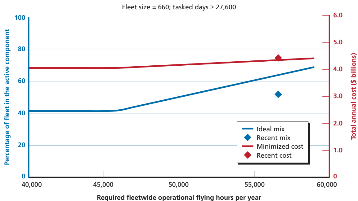
Figure C.4 Cost-Minimizing Force Mixes with Varying Operational Demand, F-16s
