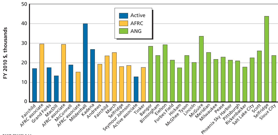
Figure B.14 Average Cost per Flying Hour, KC-135 Wings
