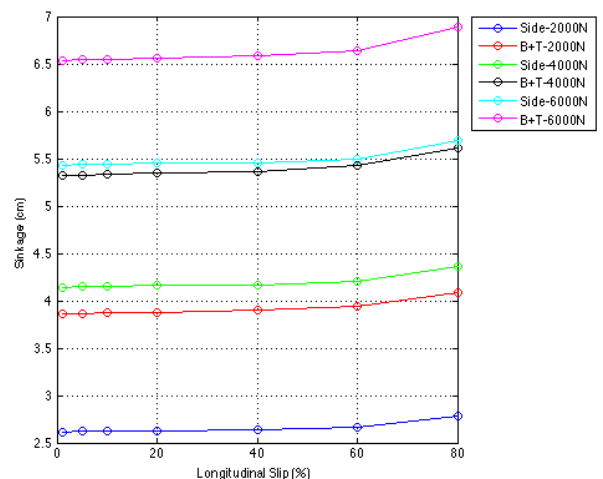
Fig. 25: Sinkage as a function of slip for different normal loads at zero slip angle
