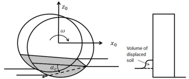
Fig. 11: Representation of the bulldozing force [8]
