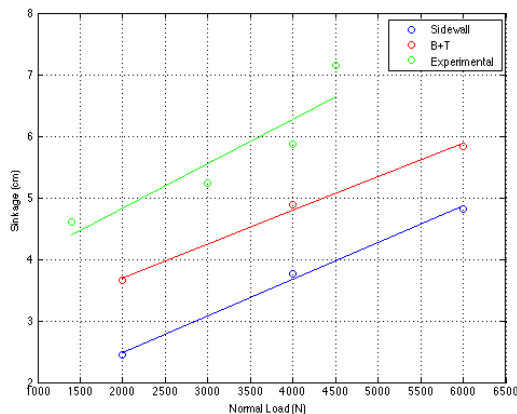
Fig. 21: Sinkage as a function of normal load for the dynamic loading case. Note that the simulation results are obtained using a Sandy Loam (11% moisture content), while the experimental data is obtained using a Silky Sand (~2% moisture content)
