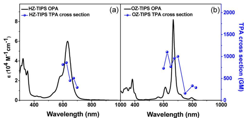
Figure 9 OPA (black solid line and left vertical axis) and TPA spectra (blue symbols and right vertical axis) of (a) HZ-TIPS and (b) OZTIPS in chloroform. TPA spectra are plotted at \lambda_{\text{ex}}/2 .
