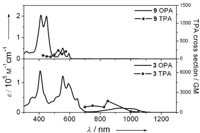
Figure 7 One- (OPA) and two-photon absorption (TPA) spectra of compounds 9 (top) and 3 (bottom) in CH 2 Cl 2 . TPA spectra are plotted at \lambda_{ex}/2 .
