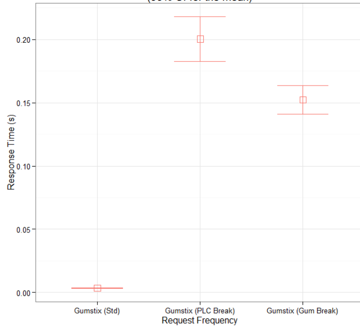
Average Return Times for HAP Standard Workload (99% CI for the mean)
