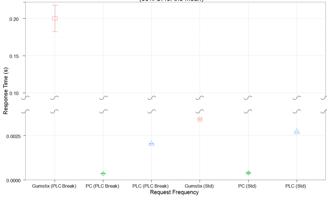
Average Return Times for HAP Standard Workload (99% CI for the mean)
