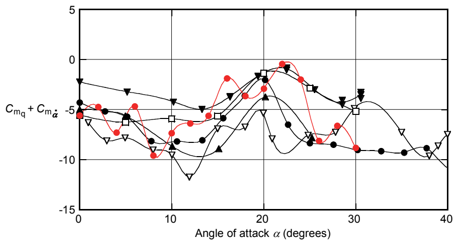
Figure 21. C_{mq} + C_{m\dot{\alpha}} vs \alpha for SDMs for different investigations.
