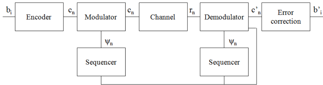
Figure 2.4: Early AFH system [21].
