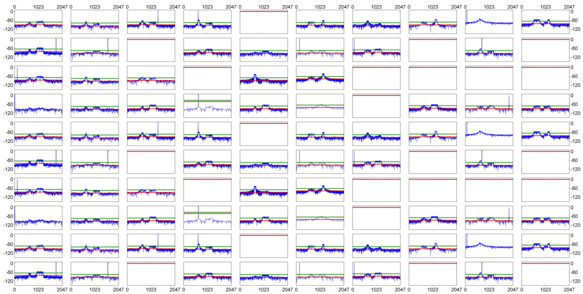
Figure A.7: DYSE-generated RF spectrum map #7.
