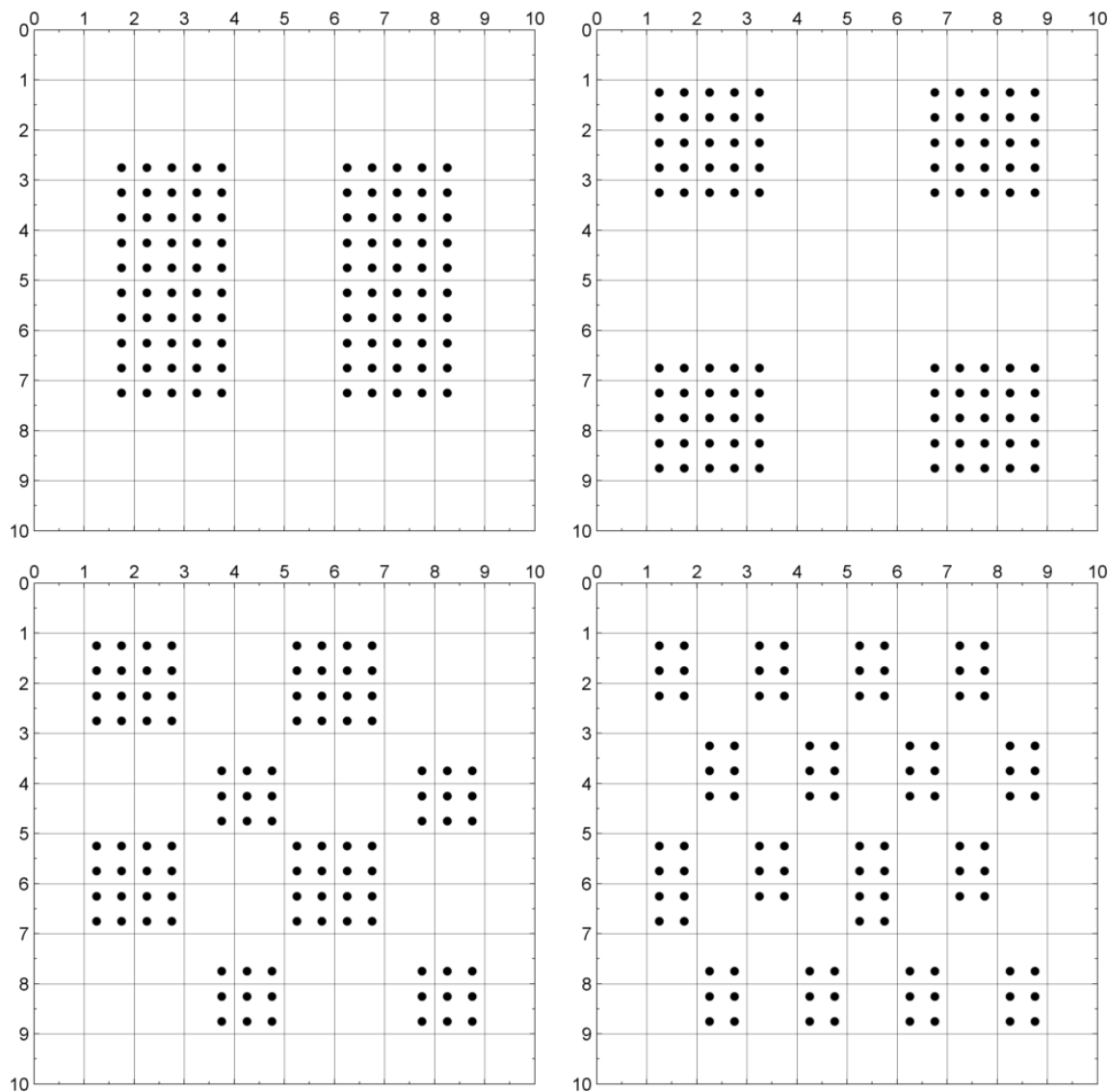
Figure 3.3: Baseline receiver configurations.
