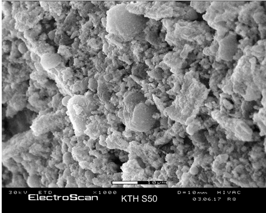
Figure L.31: Al(50nm)/Ag 2 MoO 4
