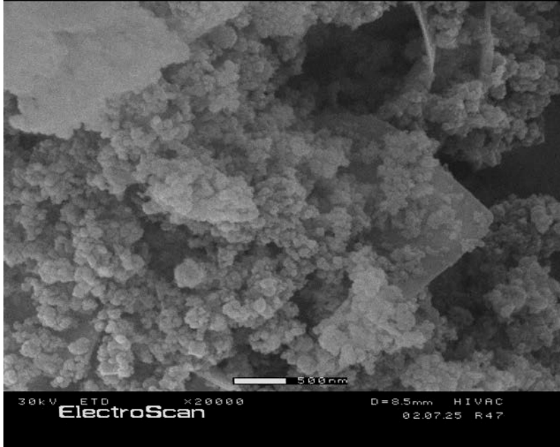
Figure L.23: Al(50nm)/MoO 3 (45nm)
