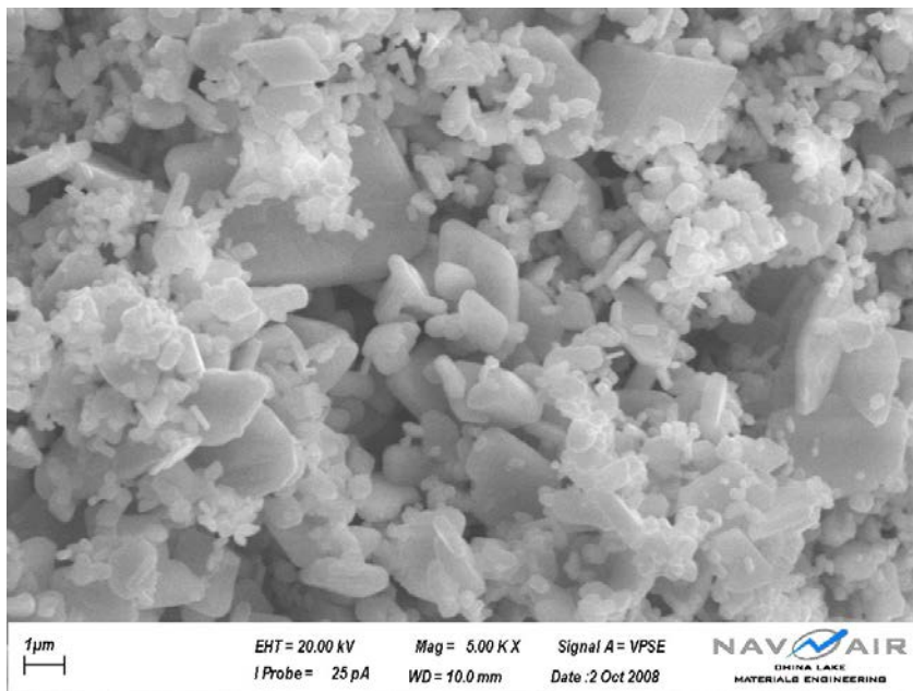
Figure L.18: NAVAIR's \text{Ag}_2\text{O}
