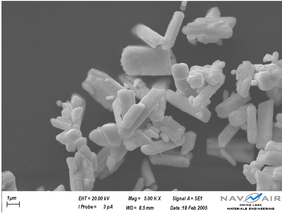
Figure L.8: Skylighter's \text{Bi}_2\text{O}_3
