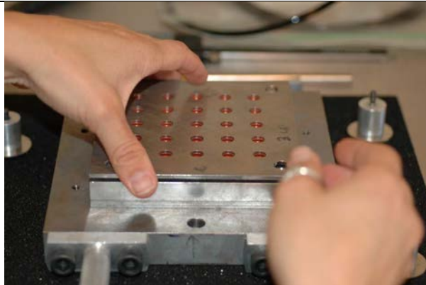
Figure 10: The Support Cup Holder Is Put In Place
