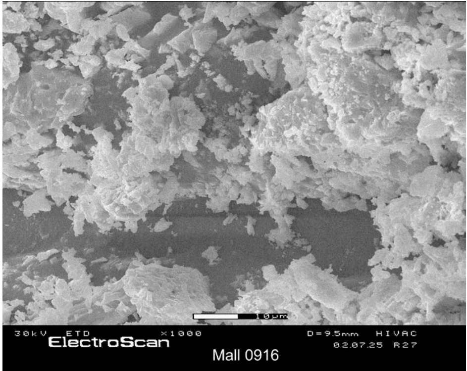
Figure L.11: Mallinkrodt's \text{MoO}_3
