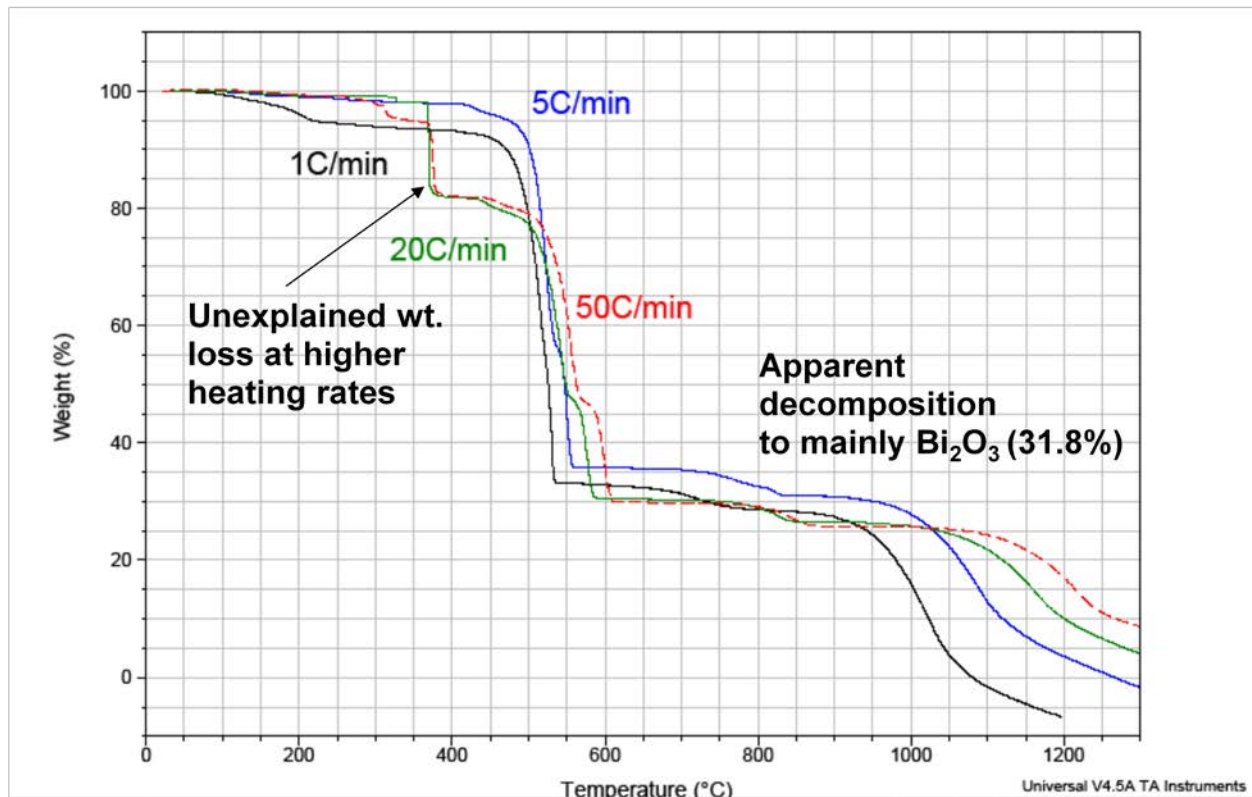
Figure H.1: TGA of Bi(IO 3 ) 3 Oxidizer
