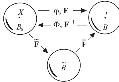
Figure 1. Mappings among reference, intermediate, and current configurations of a deformable body.
