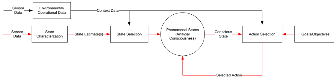
Figure 14. Bottom-up Attention Process in CASE
