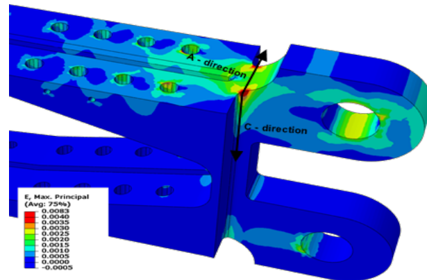
Figure 18. Model of Wing Spar Attachment Lug
