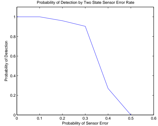
Fig. 4. Probability of detection as the error rate for the two state CBRN sensor grows. Reported values correspond to zero observed false alarms.
