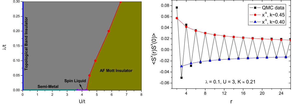
Figure 6: Left hand side (LHS): A plot of the phase diagram of the Kane-Mele-Hubbard model from our QMC simulations. The magnetic phase boundary is marked. The line of \lambda = 0 corresponds to the case of pure Hubbard model in the honeycomb lattice that was simulated in Ref. [48] by Meng et al. . Right hand side (RHS): The two-point equal-time spin correlation function \langle G | S_x(\vec{r}) S_x(\vec{r}') | G \rangle along the zig-zag edge with \lambda = 0.1 and U = 3 . The length of the zig-zag edge is 2 \times 34 and the width of the ribbon is 4. Because the zig-zag edge contains the sites of both A and B sub-lattices, the fitted decay powers are slightly different. We use their average value to obtain the Luttinger parameter K \approx 0.21 .
