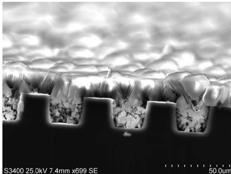
Figure 6. Picture was taken at S.M.A.R.T. Lab and is a close-up image of the LiF powder-packed trench perforations. The powder has been physically pressed into the 30\ \mu\text{m} diameter by 20\ \mu\text{m} deep holes with an evaporated LiF cap film [18]. ©2009 with permission from Elsevier.
