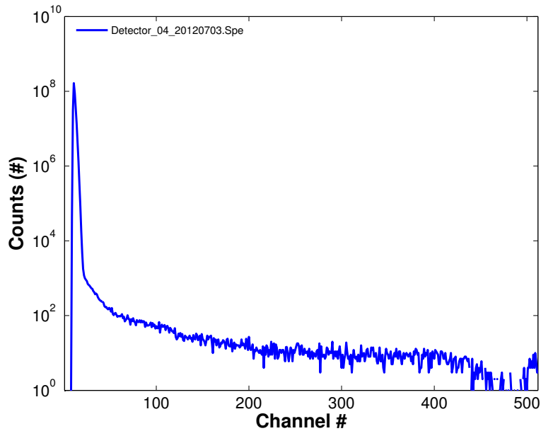
Figure 63. 12 hour test of detector 04 in the graphite pile, with Cd. Comparing this figure to Fig. 62, the reduction in signal (two orders of magnitude), is proof that the detectors have a good response to thermal neutrons.
