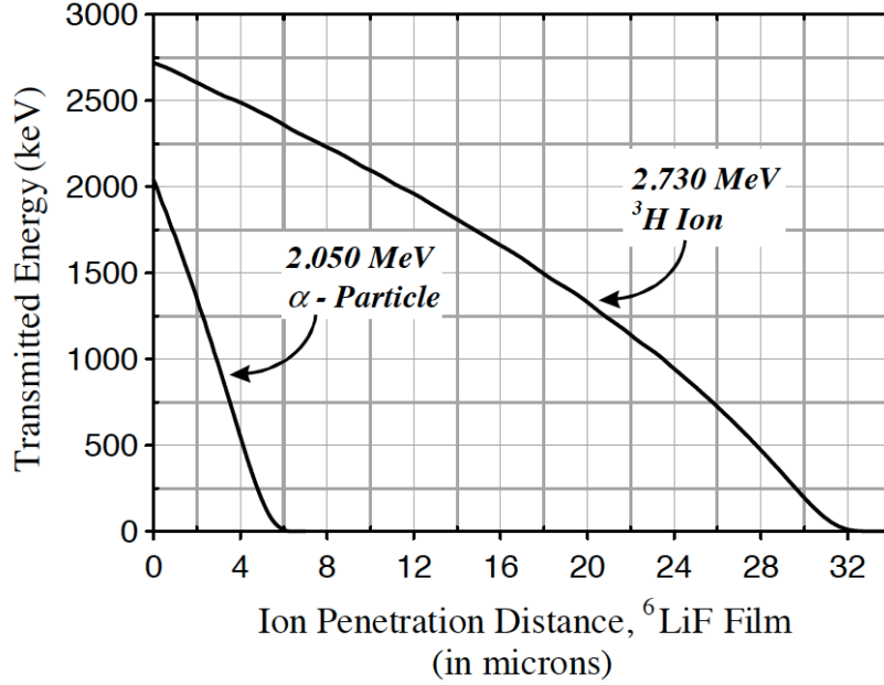
Figure 15. Energy deposited into the detector is the original particle energy minus the energy lost through self-absorption. Shown are the particle energies remaining from the {}^6\text{Li}(n,\alpha){}^3\text{H} reaction as a function of transit distance through LiF [17]. ©2003 with permission from Elsevier.
