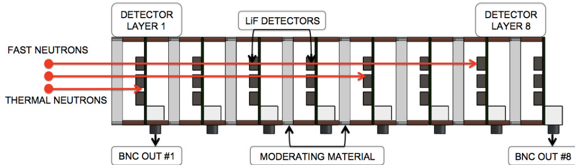
Figure 24. Model of the eight-layer spectrometer created in Solidworks ® . The model shows nine detectors in each layer (3 x 3). The nine-detector design was the original concept to achieve higher detection efficiency with each detection layer, however, only one detector was mounted in the center of each detector layer due to lack of operational detectors.
