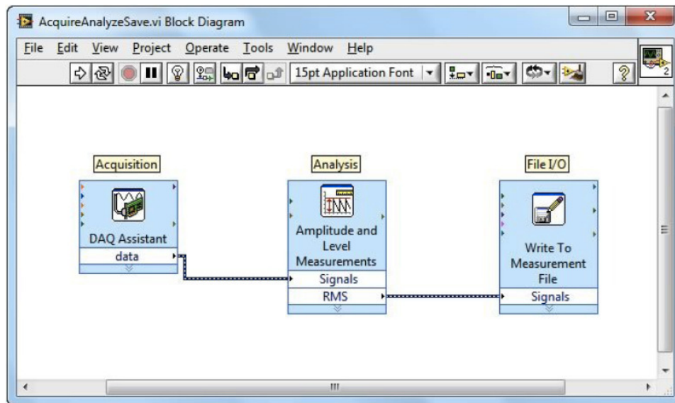
Figure 42. LabVIEW ® program for data acquisition, analysis and writing to a file. Data originates in the acquisition function and then flows intuitively to the analysis and storage function through wires.
