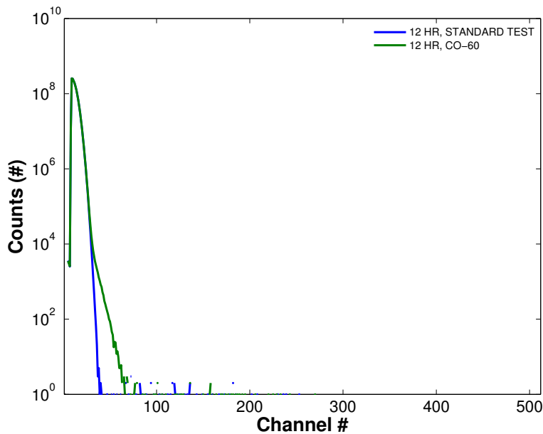
Figure 67. Two tests conducted with detector 06 removed and isolated from the graphite pile. The first test was conducted with the Co-60 source present and the second was performed with the source removed. The blue line represents only background and the green line represents the Co-60 source present. Test was conducted for 12 hours.
