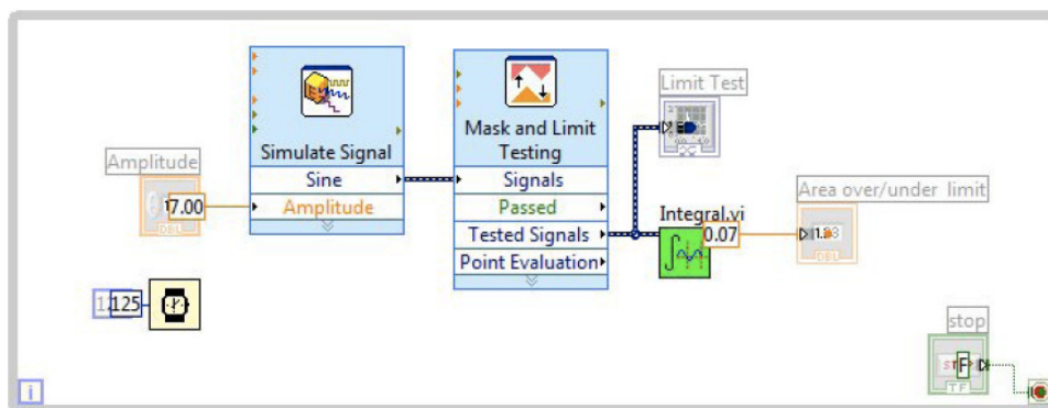
Figure 43. LabVIEW ® interactive debugging environment allows visualization of data values as they pass from function to function along wires, reporting datum as they are analyzed real-time. This option is known as execution highlighting and it provides an intuitive way to understand the execution order of G code.
