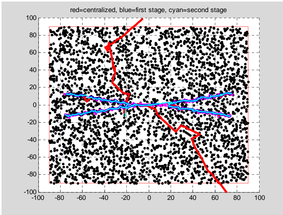
Figure 3.1: Crossing target trajectories (magenta), contact data (black), single-stage adaptive tracking (red), first-stage tracking (blue), track-adapt-track (cyan).
