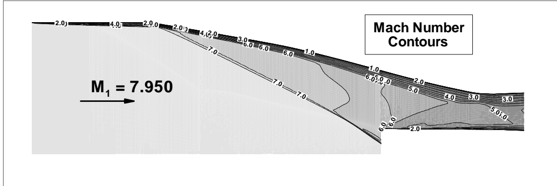
Figure 19: Symmetry plane Mach number contours in the RESTM12 inlet at M_0 = 10 .
