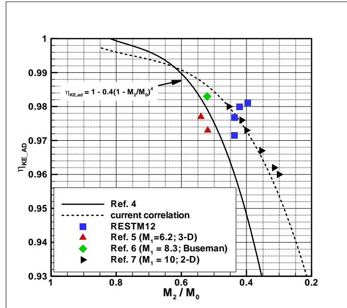
Figure 4: Inlet efficiency data compared to a number of correlations.
