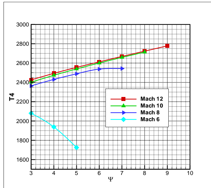
Figure 14: Static temperature at the entrance to the nozzle.
