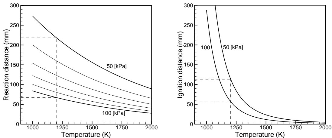
Figure 16: Ignition and reaction lengths of hydrogen assuming a combustor velocity of 2400 m/s.
