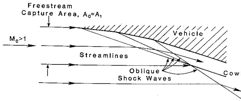
Figure 5: External compression inlet (Heiser and Pratt 3 ).
