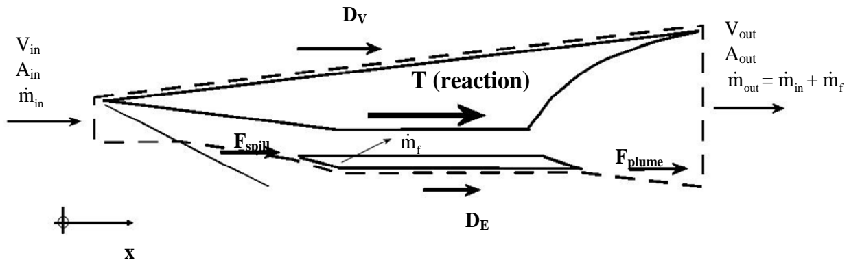
Figure 9: Schematic of control volume used for scramjet performance analysis.
