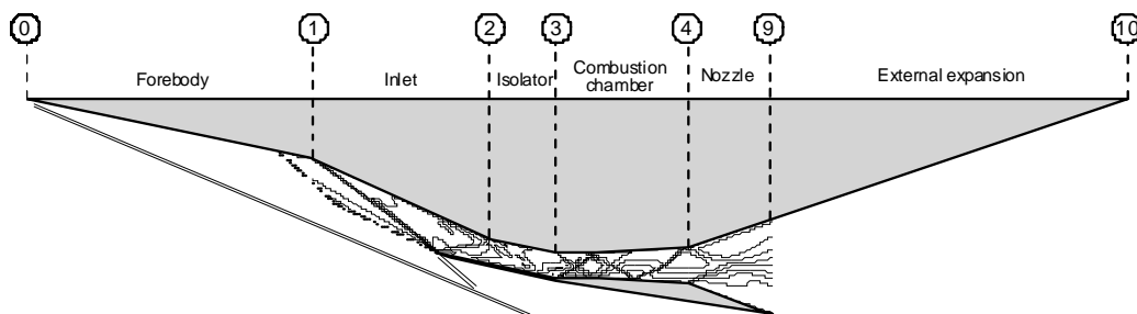
Figure 2: Flow stations in a scramjet engine.
