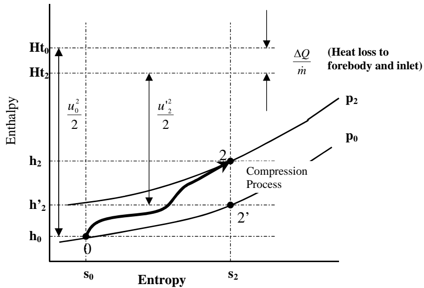
Figure 3: Mollier diagram of inlet compression process.
