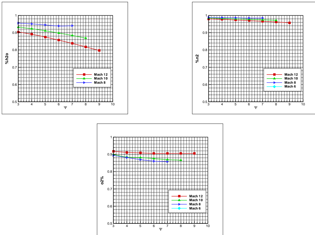
Figure 15: Species mole fractions at the entrance to the nozzle.
