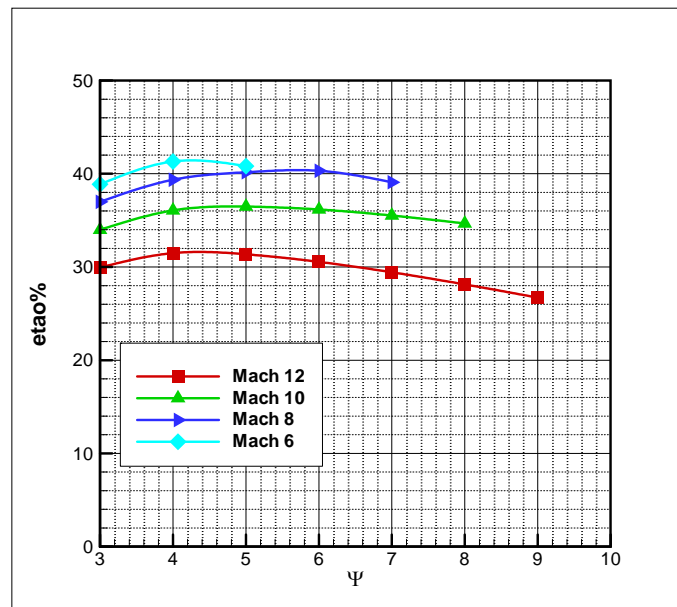
Figure 13: Overall scramjet cycle efficiency.
