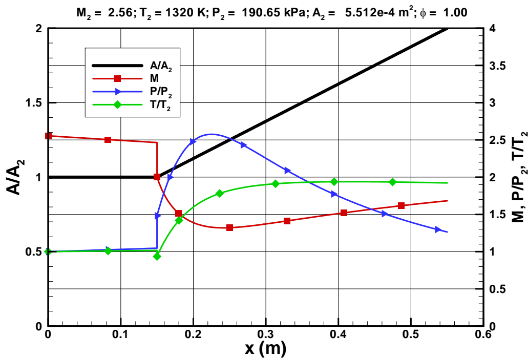
Figure 12: Example results of the combustor analysis.
