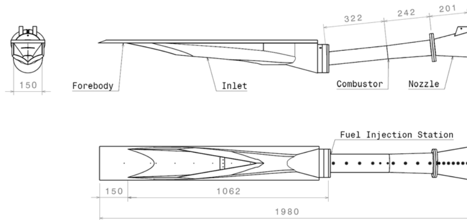
Figure 18: Schematic of the RESTM12 engine model (dimensions in mm).
