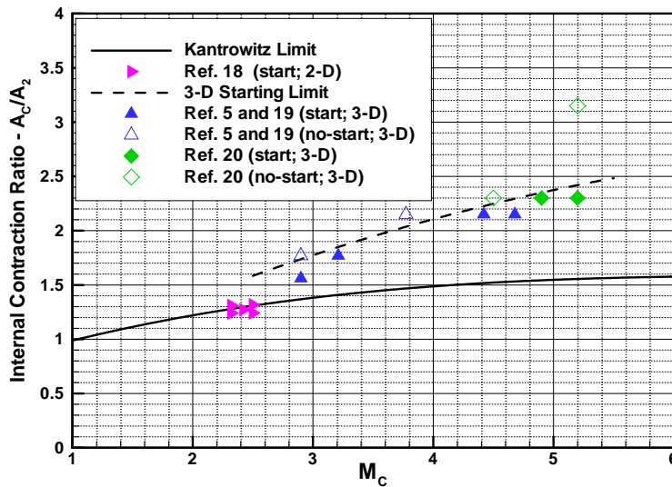
Figure 17: Experimental data on starting limits for 2-D and 3-D inlet geometries.
