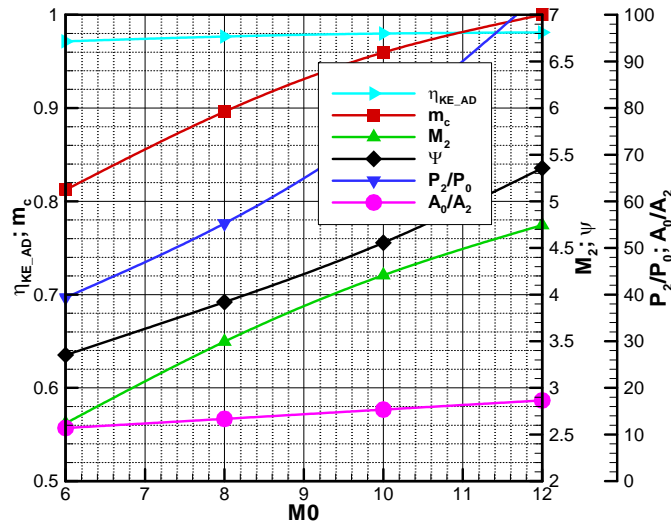
Figure 20: RESTM12 Inlet capability parameters.
