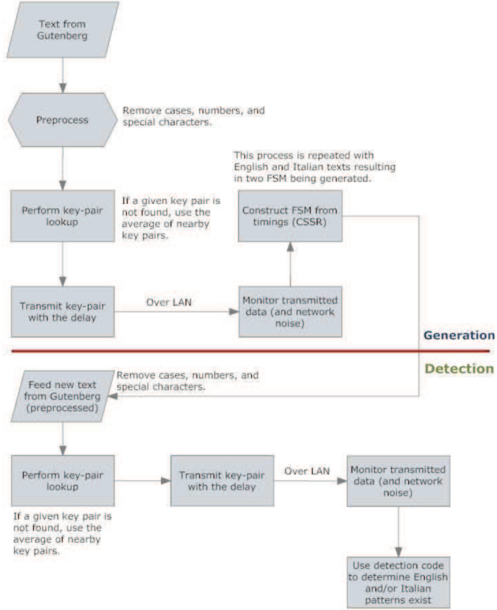
Figure 2.1: Language Data-Flow
