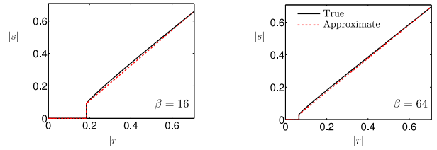
Fig. 1. Gradient magnitude “shrinkage” function for \alpha = 2/3 and different values of \beta . We show the true function, as well as the thresholded-linear approximation used in our implementation.
