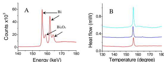
Figure 3. XPS spectrum of surface oxidized bismuth nanoparticles (A); DSC curves of indium nanoparticles immobilized on aluminum by biotin-avidin interaction (B).
