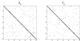
Fig. 1. Sparse Kronecker matrix representation. Left panel: left Kronecker factor. Right panel: right Kronecker factor.
