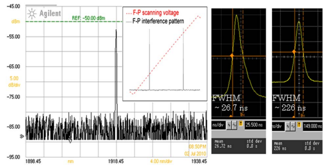
Fig. 3. (Color online) Spectrum and typical pulse shapes of single-frequency Q-switched fiber laser seed.
