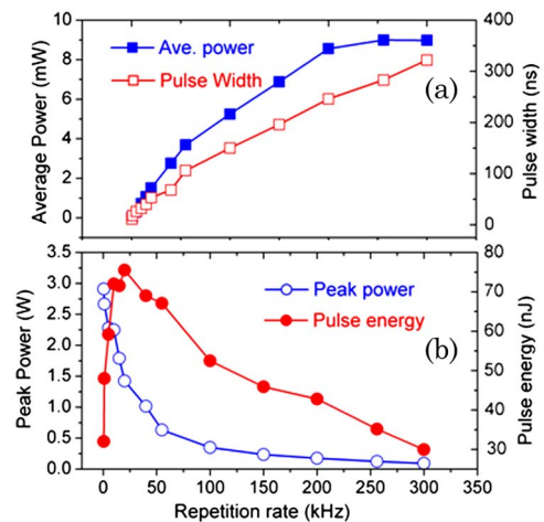
Fig. 4. (Color online) (a) Average power and pulse width, and (b) peak power and pulse energy at different repetition rates when the pump power is \sim 300 mW for the Q-switched fiber laser seed.
