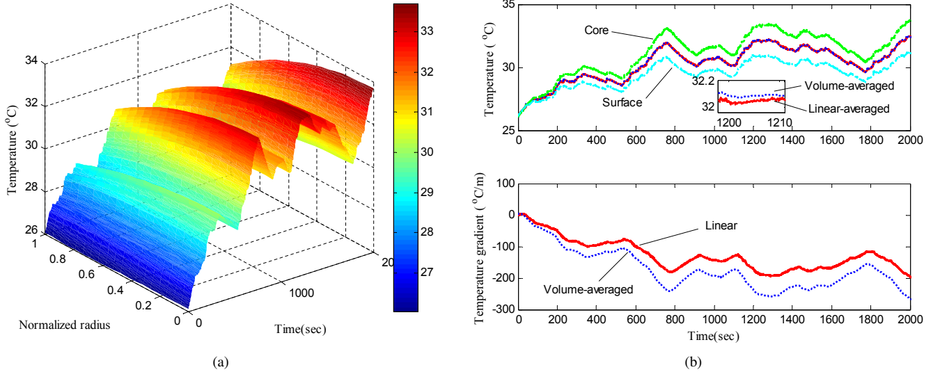
Fig. 6. (a) Expected temperature distribution along the normalized radius ( r/R ) using polynomial approximation; (b) Cell temperature (top) and temperature gradient (bottom)
