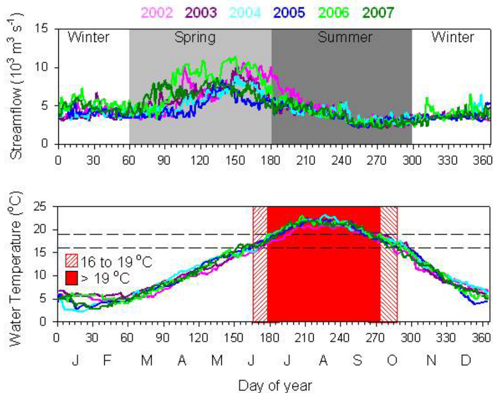
Figure 11. Seasonal and interannual variation in river flow (upper panel) and temperature (lower panel) by day of year at Bonneville Dam 2002-2007. Seasonal divisions are indicated in the upper panel, and temperature regimes in the lower panel. Data courtesy of Columbia River Data Access in Real Time (CRDART 1995).
