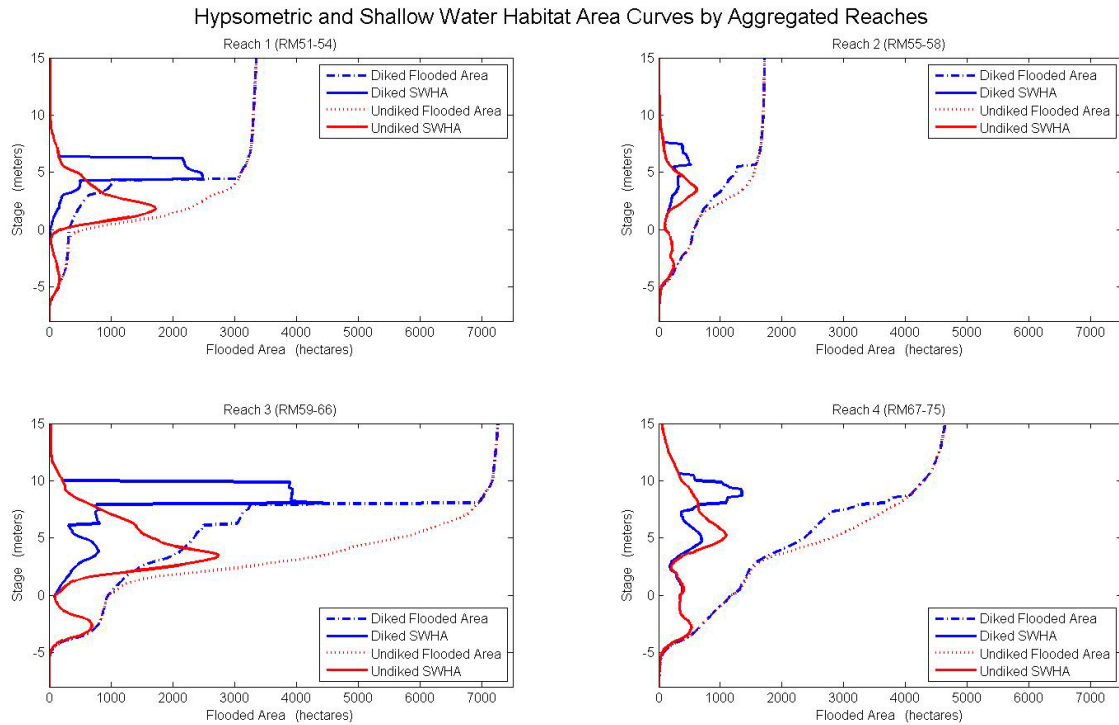
Figure 4. Sub-reach hypsometric and shallow-water habitat area (SWHA) vs. elevation curves for the Eagle Cliff to Kalama reach (rkm 83-120), for diked and undiked topography.
