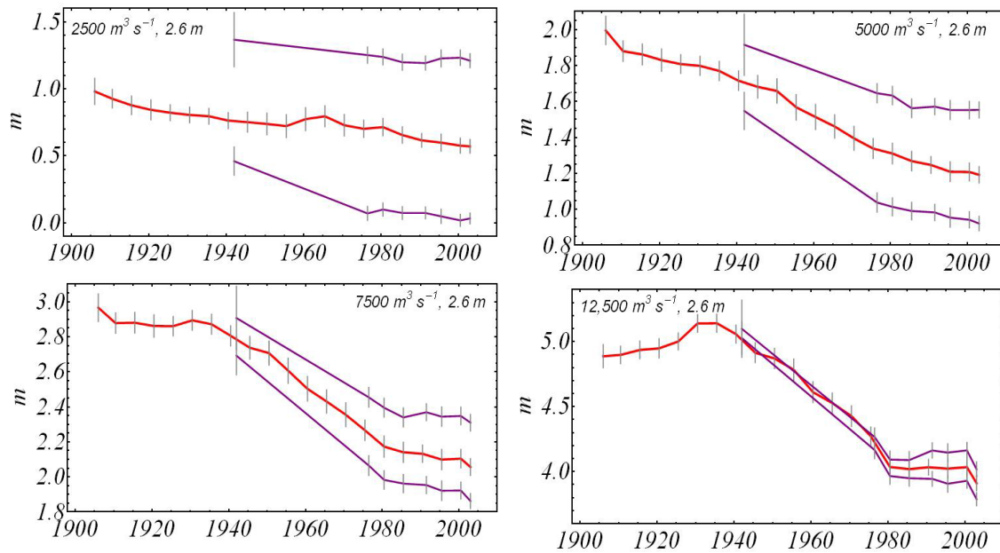
Figure 1. Each panel shows higher high water (upper line), mean water level (center line), and lower low water (lower line) at Vancouver, WA, in 5-year intervals. Water levels at Vancouver reflect flow levels at The Dalles of 2,500, 5,000, 7,500 and 12,500 \text{m}^3\text{s}^{-1} , all for a tidal range of 2.6 m at Tongue Pt. Gray bars indicate 95% CIs.
