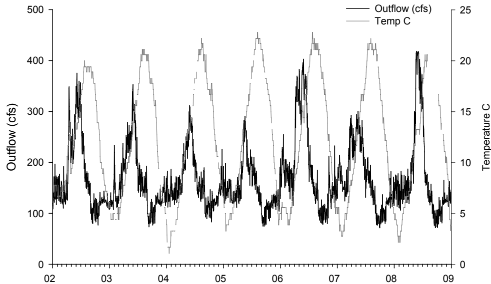
Figure 27. River discharge and temperature at Bonneville Dam, 2002-2008. Data from US Geological Survey (USGS 2006).
