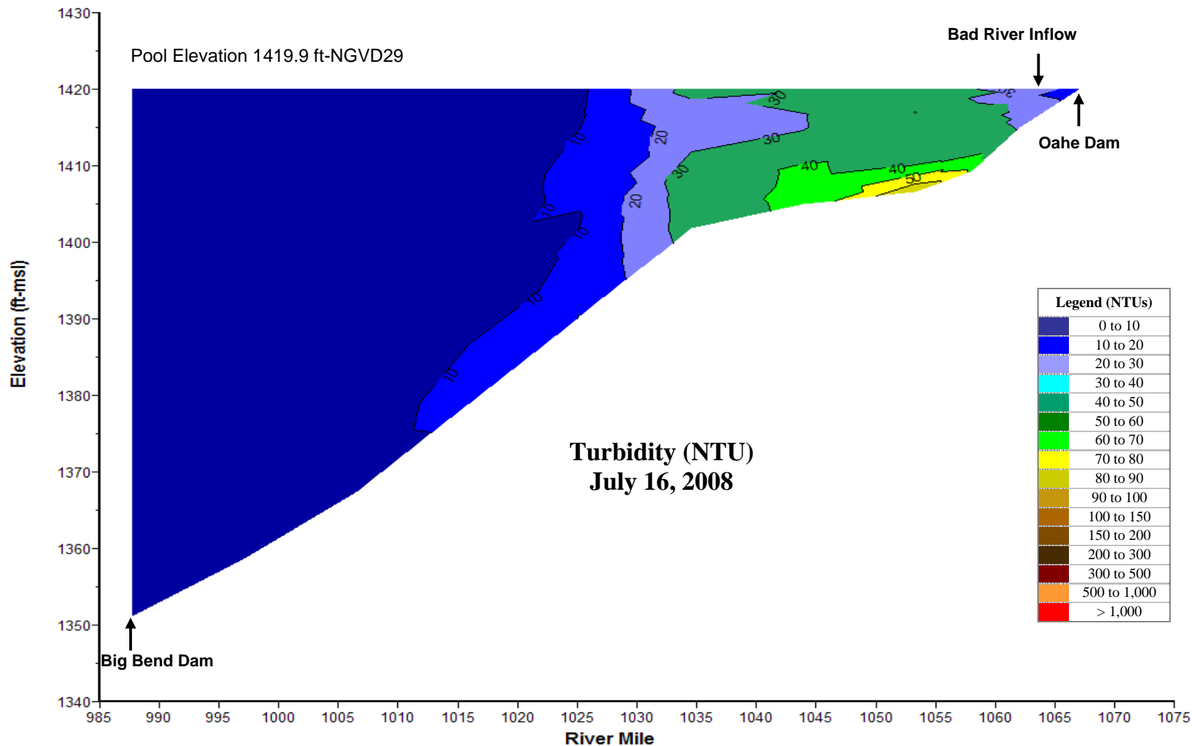
Plate 26. Longitudinal turbidity (NTU) contour plot of Lake Sharpe based on depth-profile turbidity levels measured at sites BBDLK0987A, BBDLK1004DW, BBDLK1020DW, BBDLK1036DW, BBDLK1055DW, and OAHPP1 on July 16, 2008.
