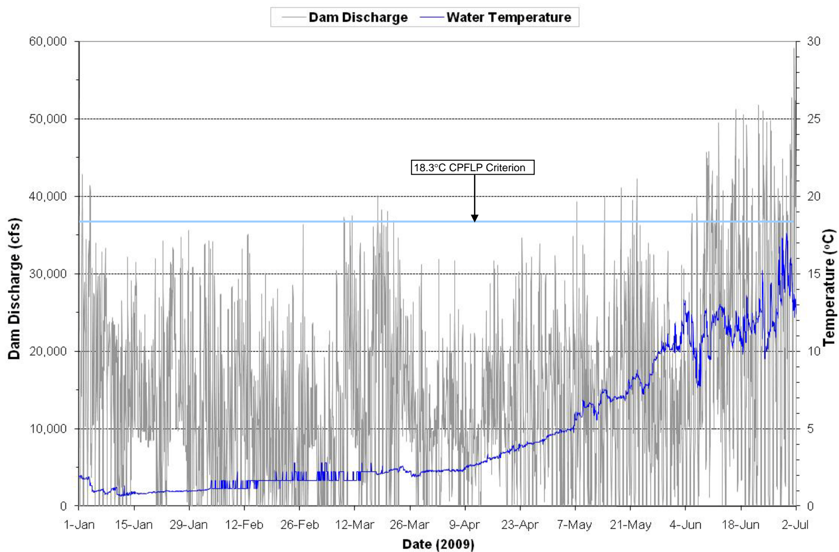
Plate 39. Hourly discharge and water temperature monitored at the Oahe powerplant on water discharged through the dam during the period January through June 2009.
