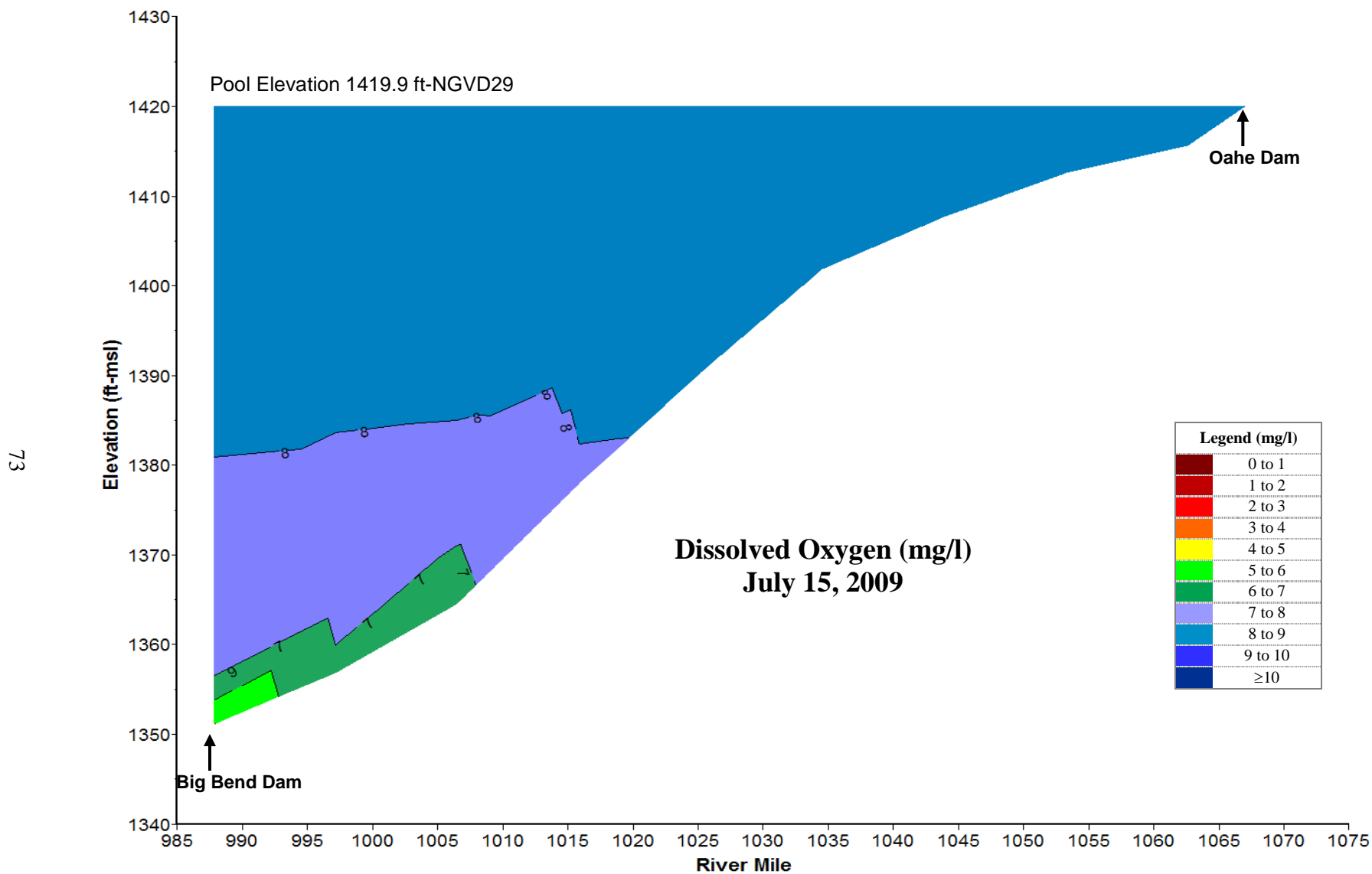
Plate 18. Longitudinal dissolved oxygen (mg/l) contour plot of Lake Sharpe based on depth-profile dissolved oxygen concentrations measured at sites BBDLK0987A, BBDLK1004DW, BBDLK1020DW, BBDLK1036DW, BBDLK1055DW, and OAHPP1 on July 15, 2009.
