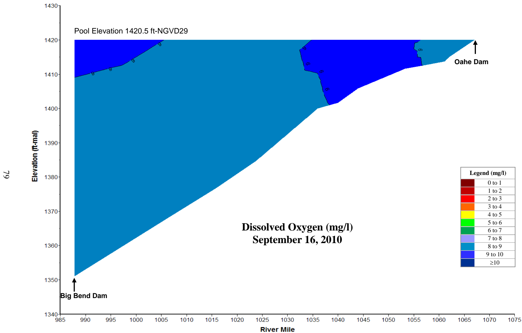
Plate 24. Longitudinal dissolved oxygen (mg/l) contour plot of Lake Sharpe based on depth-profile dissolved oxygen concentrations measured at sites BBDLK0987A, BBDLK1020DW, BBDLK1055DW, and OAHPP1 on September 16, 2010.
