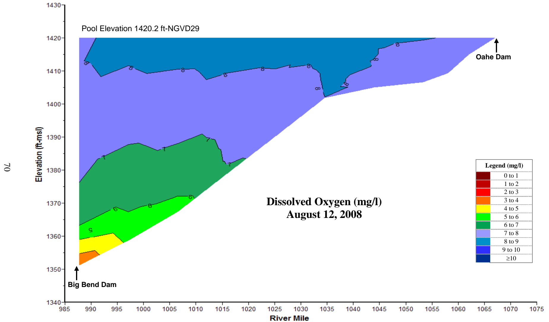
Plate 15. Longitudinal dissolved oxygen (mg/l) contour plot of Lake Sharpe based on depth-profile dissolved oxygen concentrations measured at sites BBDLK0987A, BBDLK1004DW, BBDLK1020DW, BBDLK1036DW, BBDLK1055DW, and OAHPP1 on August 12, 2008.
