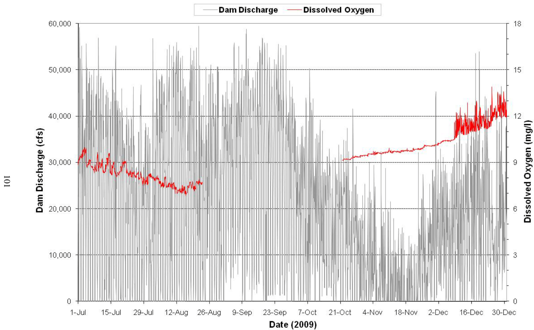
Plate 46. Hourly discharge and dissolved oxygen monitored at the Oahe Powerplant on water discharged through the dam during the period July through December 2009.
