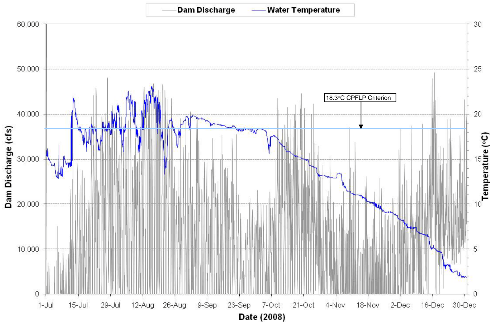
Plate 38. Hourly discharge and water temperature monitored at the Oahe powerplant on water discharged through the dam during the period July through December 2008.
