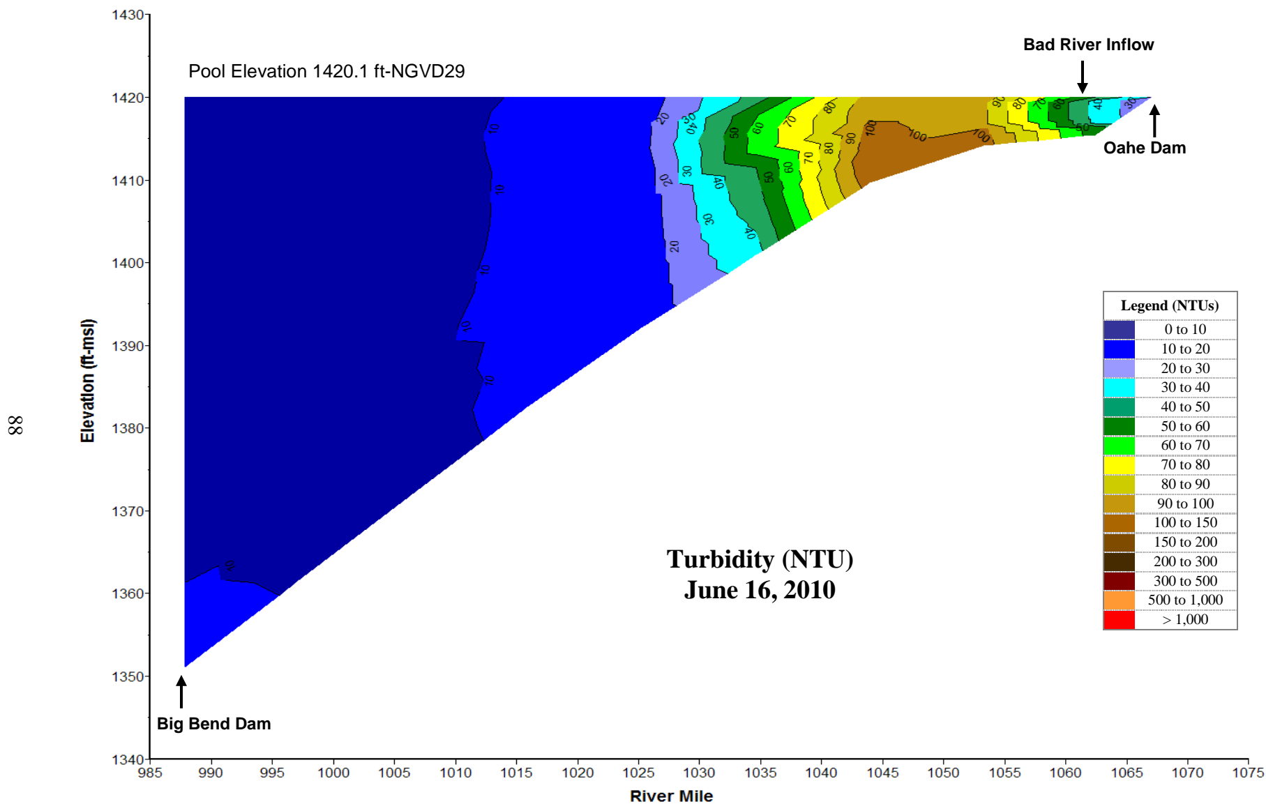
Plate 33. Longitudinal turbidity (NTU) contour plot of Lake Sharpe based on depth-profile turbidity levels measured at sites BBDLK0987A, BBDLK1020DW, BBDLK1055DW, and OAHPP1 on June 16, 2010.
