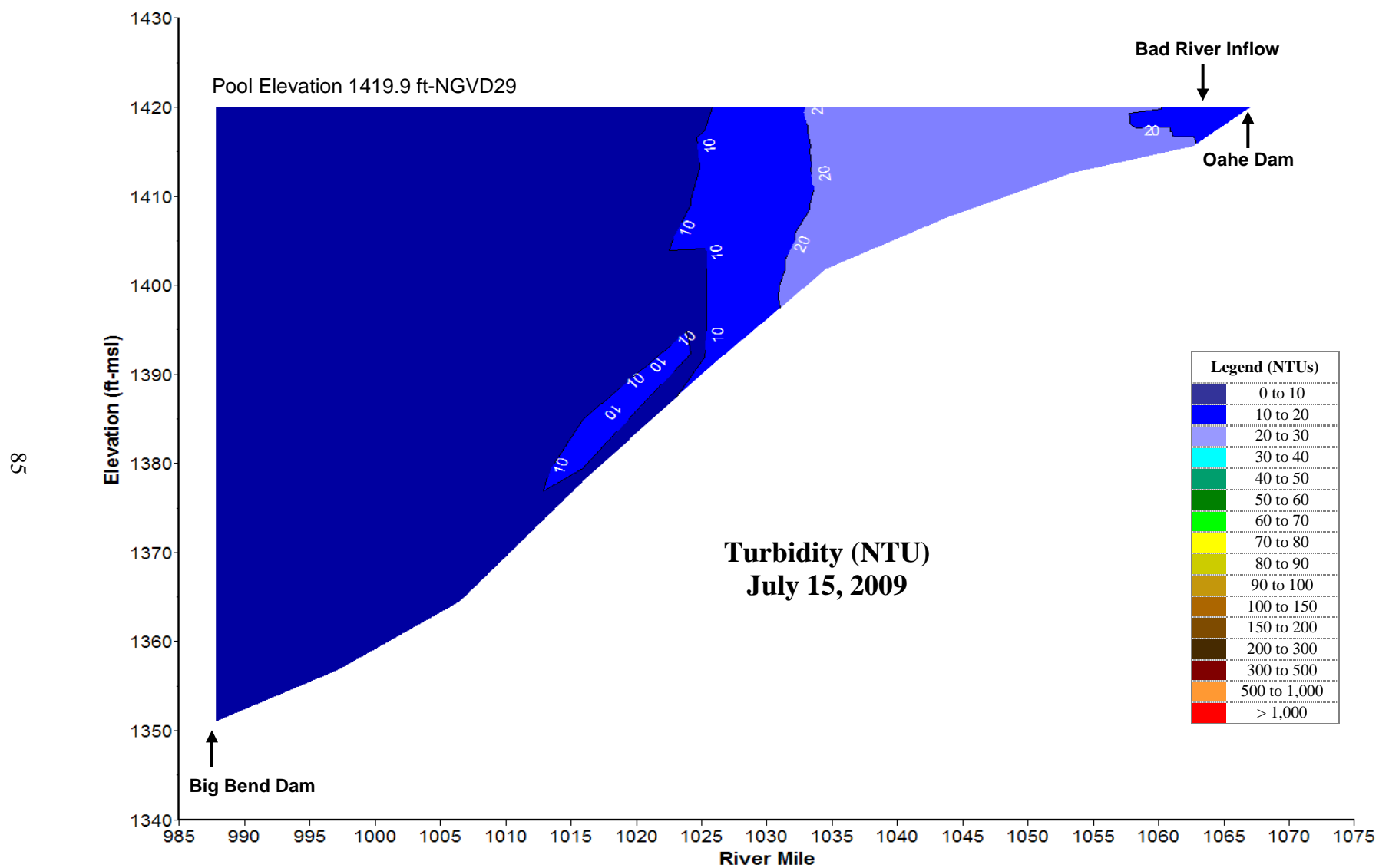
Plate 30. Longitudinal turbidity (NTU) contour plot of Lake Sharpe based on depth-profile turbidity levels measured at sites BBDLK0987A, BBDLK1004DW, BBDLK1020DW, BBDLK1036DW, BBDLK1055DW, and OAHPP1 on July 15, 2009.
