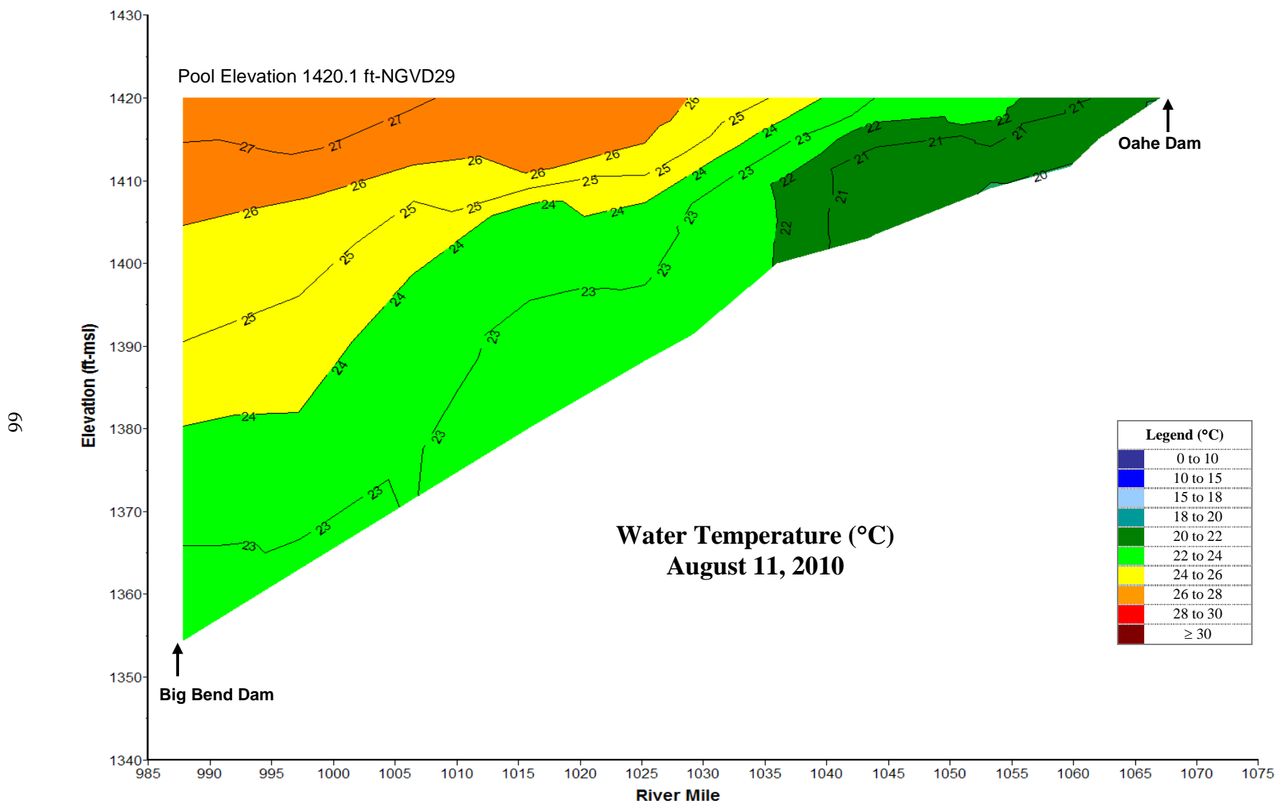
Plate 11. Longitudinal water temperature (°C) contour plot of Lake Sharpe based on depth-profile water temperatures measured at sites BBDLK0987A, BBDLK1020DW, BBDLK1055DW, and OAHPP1 on August 11, 2010.
