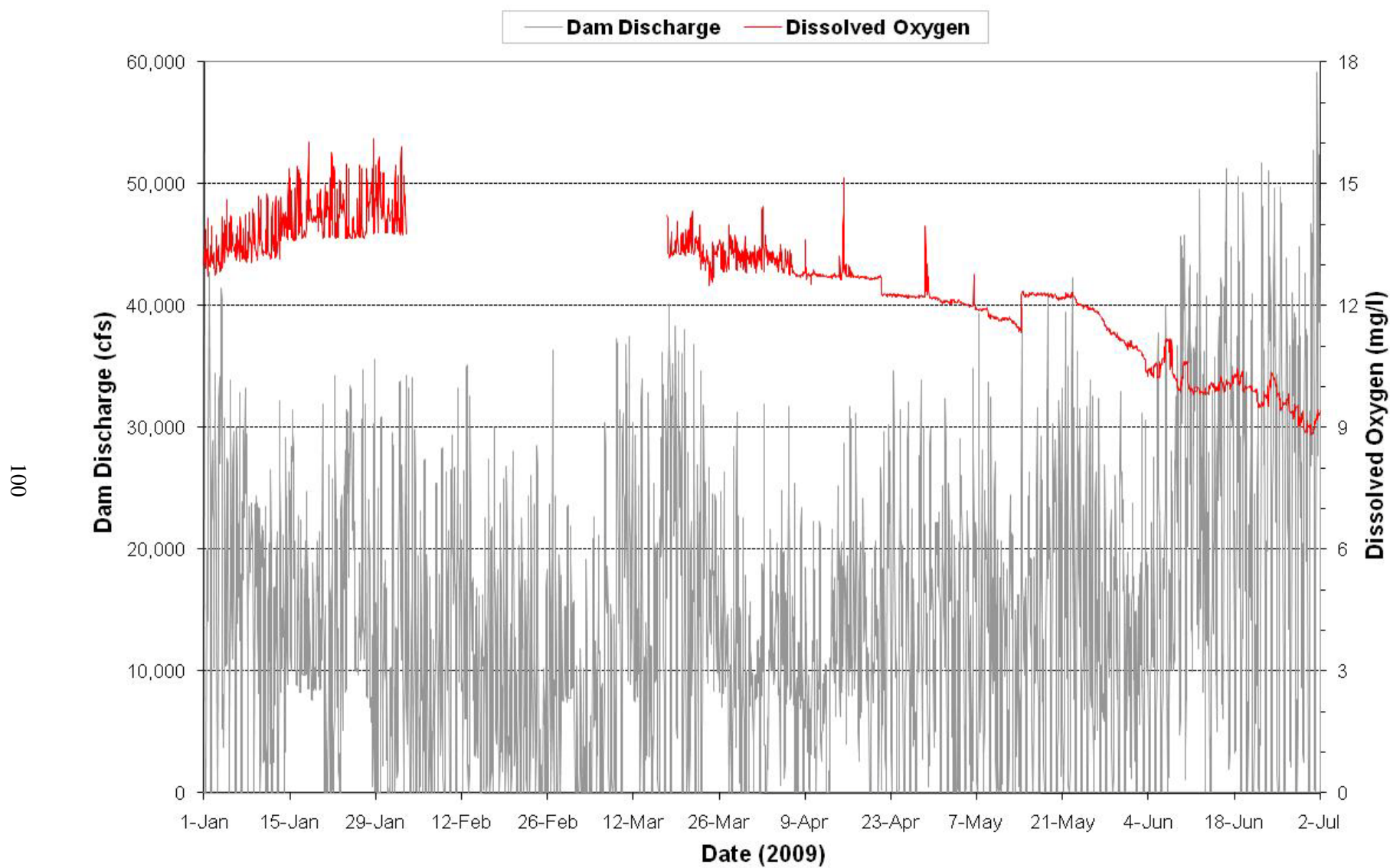
Plate 45. Hourly discharge and dissolved oxygen monitored at the Oahe Powerplant on water discharged through the dam during the period January through June 2009.
