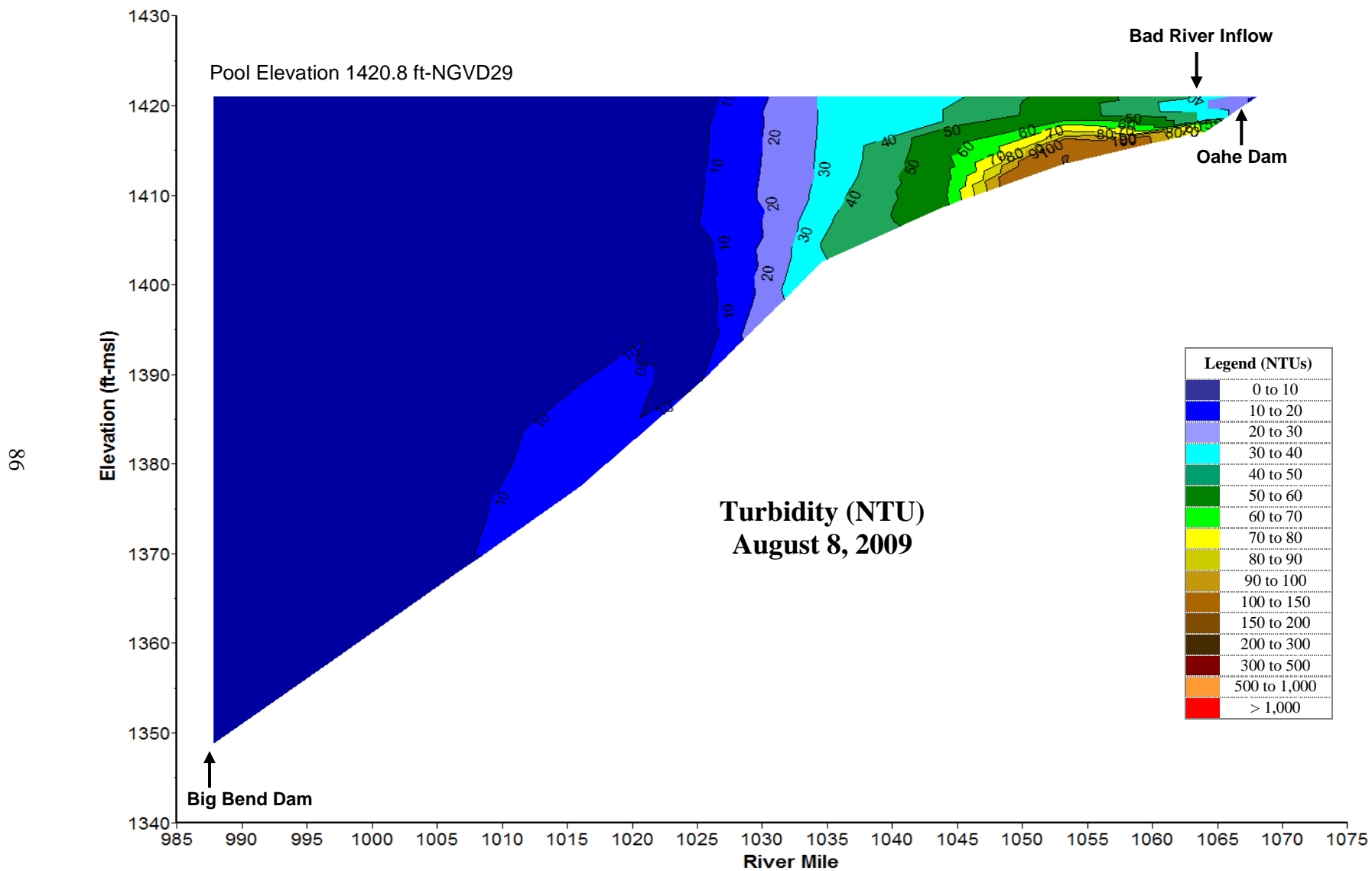
Plate 31. Longitudinal turbidity (NTU) contour plot of Lake Sharpe based on depth-profile turbidity levels measured at sites BBDLK0987A, BBDLK1004DW, BBDLK1020DW, BBDLK1036DW, BBDLK1055DW, and OAHPP1 on August 8, 2009.
