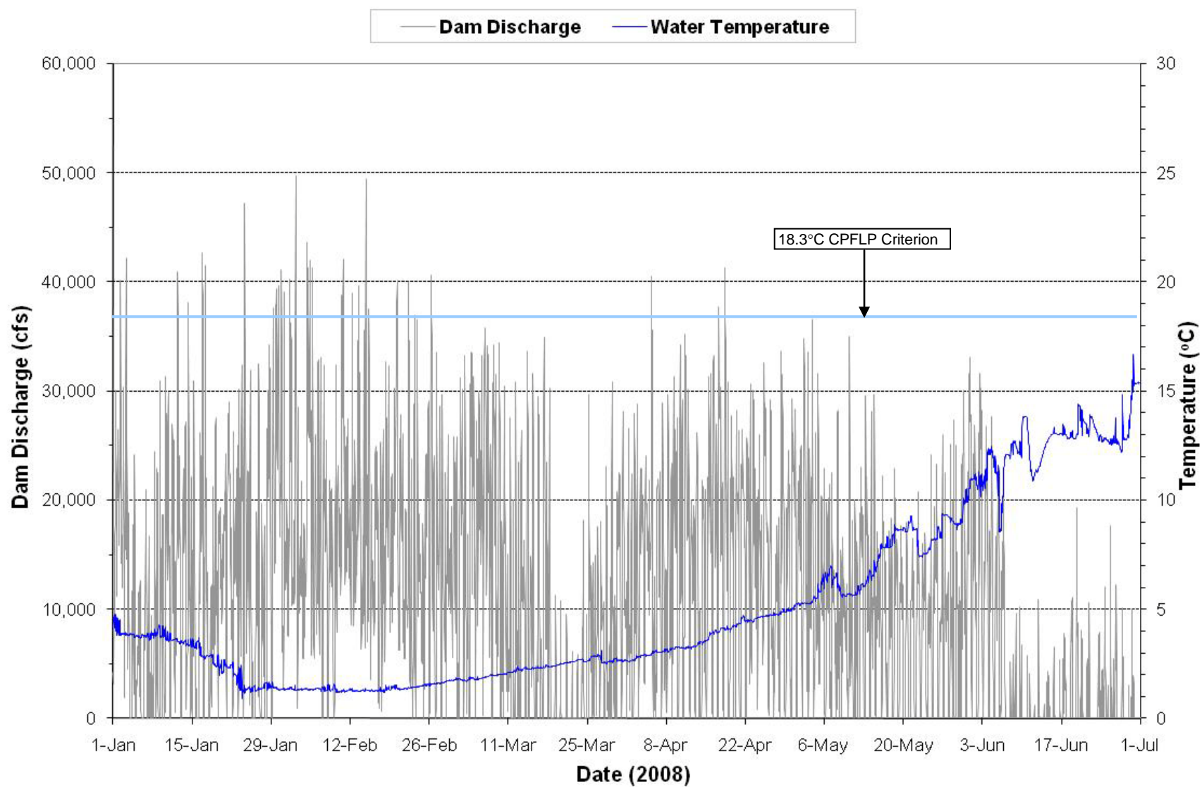
Plate 37. Hourly discharge and water temperature monitored at the Oahe powerplant on water discharged through the dam during the period January through June 2008.
