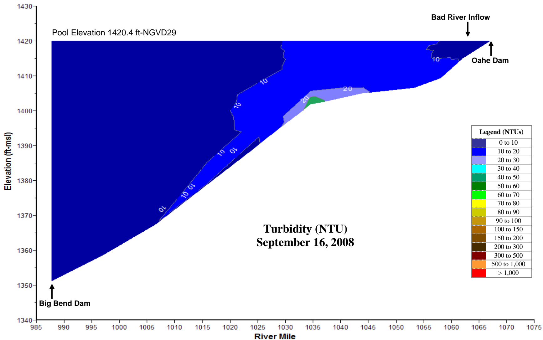
Plate 28. Longitudinal turbidity (NTU) contour plot of Lake Sharpe based on depth-profile turbidity levels measured at sites BBDLK0987A, BBDLK1004DW, BBDLK1020DW, BBDLK1036DW, BBDLK1055DW, and OAHPP1 on September 16, 2008.
