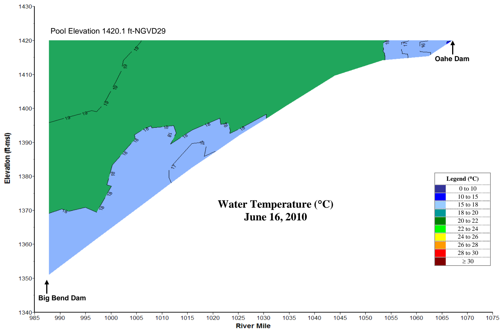
Plate 9. Longitudinal water temperature (°C) contour plot of Lake Sharpe based on depth-profile water temperatures measured at sites BBDLK0987A, BBDLK1020DW, BBDLK1055DW, and OAHPP1 on June 16, 2010.
