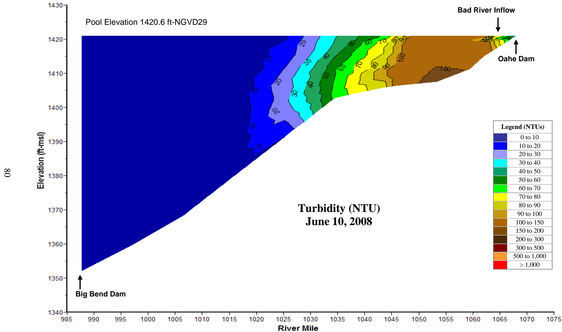
Plate 25. Longitudinal turbidity (NTU) contour plot of Lake Sharpe based on depth-profile turbidity levels measured at sites BBDLK0987A, BBDLK1004DW, BBDLK1020DW, BBDLK1036DW, BBDLK1055DW, and OAHPP1 on June 10, 2008.
