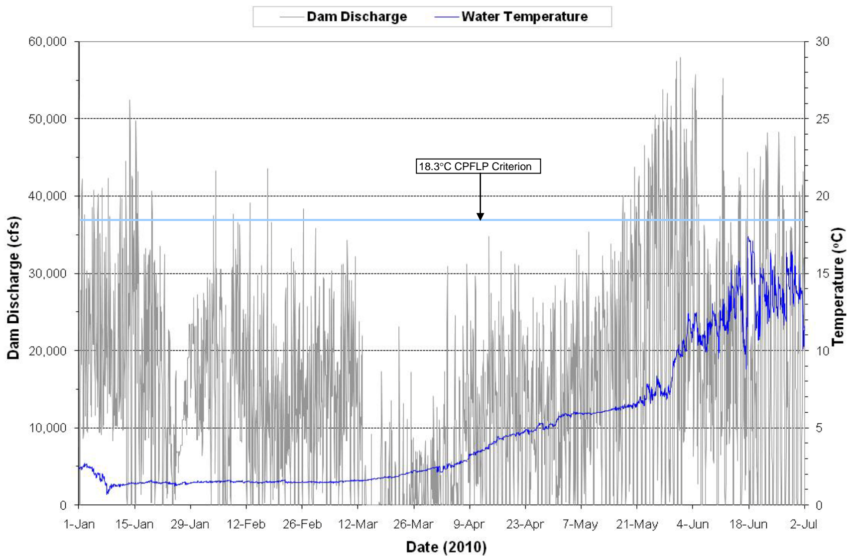
Plate 41. Hourly discharge and water temperature monitored at the Oahe powerplant on water discharged through the dam during the period January through June 2010.
