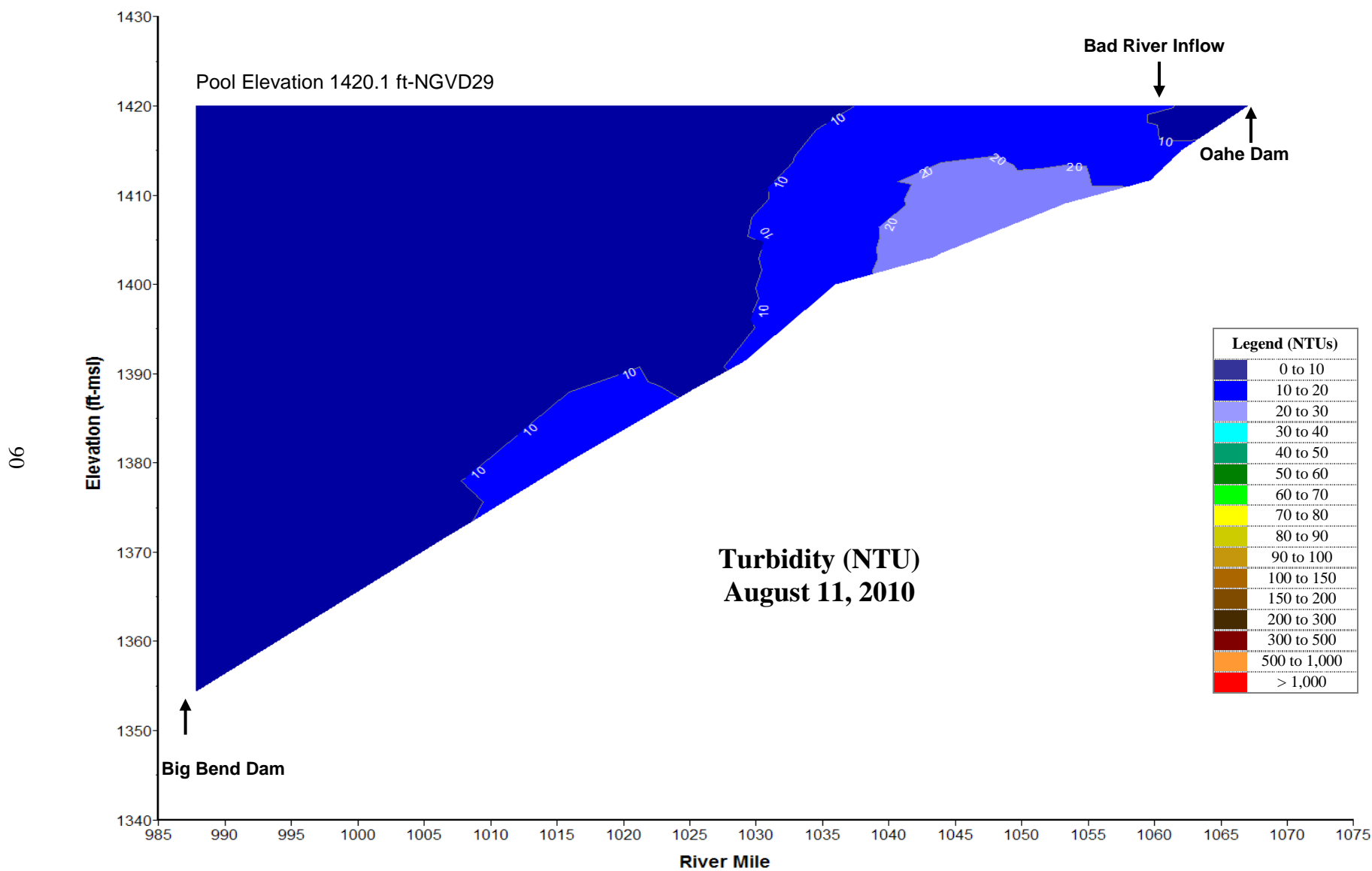
Plate 35. Longitudinal turbidity (NTU) contour plot of Lake Sharpe based on depth-profile turbidity levels measured at sites BBDLK0987A, BBDLK1020DW, BBDLK1055DW, and OAHPP1 on August 11, 2010.
