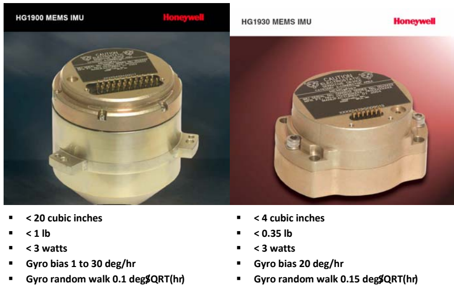
Figure 21: Honeywell MEMS IMUs (Ref. [3]).
