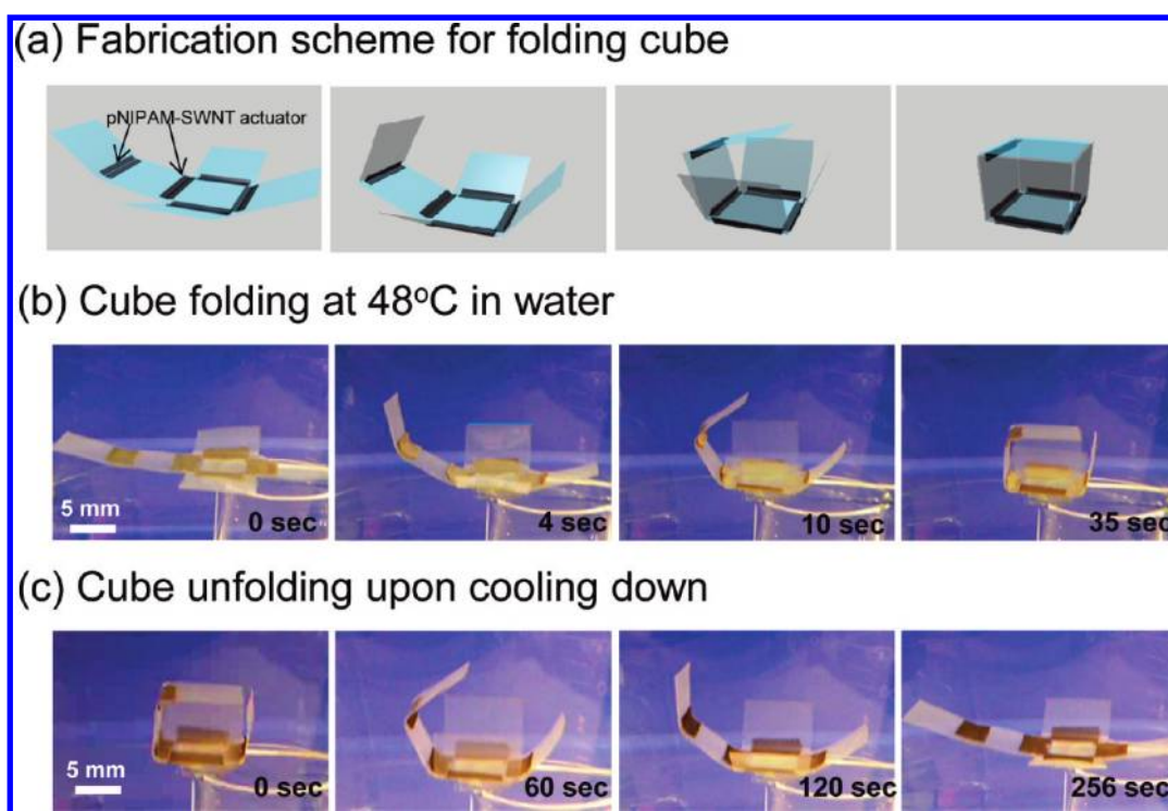
Figure 3. Programmable cubes — a folding cube based on thermal responsive actuators. (a) Fabrication scheme for folding cubes based on SWNT-pNIPAM/LDPE bilayer actuators. (b) Cube folding by thermal actuation in 48 °C water. (c) Cube reversibly unfolds by cooling down the water bath in which cube is immersed.
