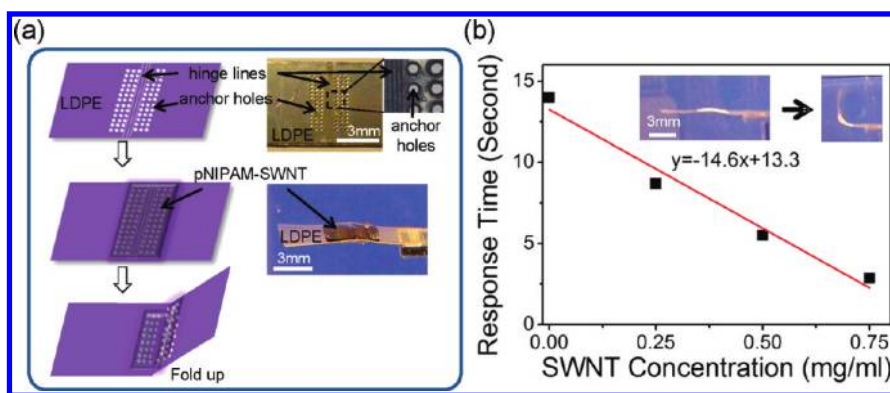
Figure 2. Fabrication scheme for making thermally responsive actuators and response time measurement. (a) Fabrication scheme for making SWNT-pNIPAM/LDPE bilayer actuators and the corresponding optical images. (b) Response time measurement by measuring the time for the actuator to reach 90° folding angle. The inset shows an optical image of a pNIPAM/LDPE actuator before (left) and right (after) folding.
