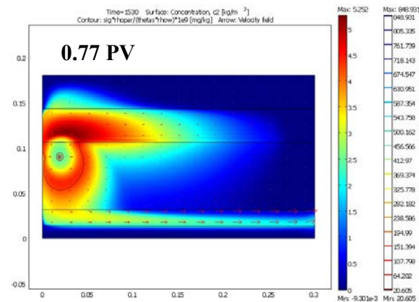
Figure 7.3.3 A comparison between experimental and modeling results of MRNIP2 transport in 2-D heterogeneous porous media at similar PV.
