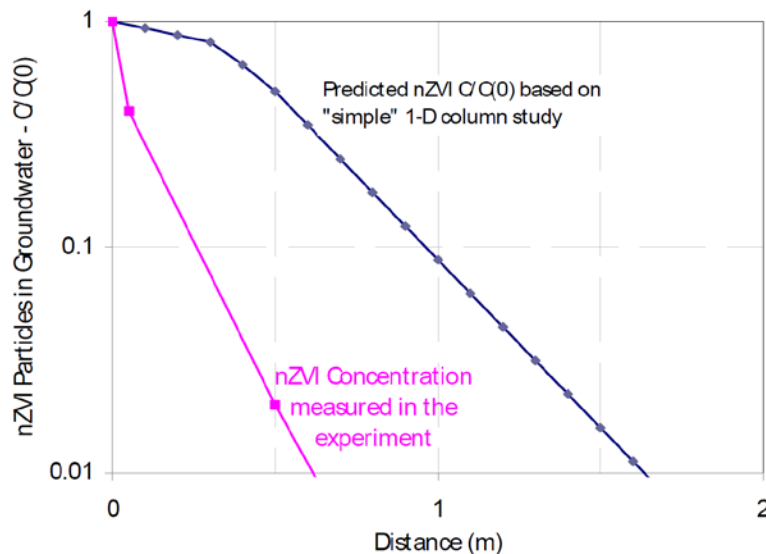
Figure 7.7.2. NZVI transport distance based on filtration models and column transport studies and transport distance measured in the field-scale experiment.
