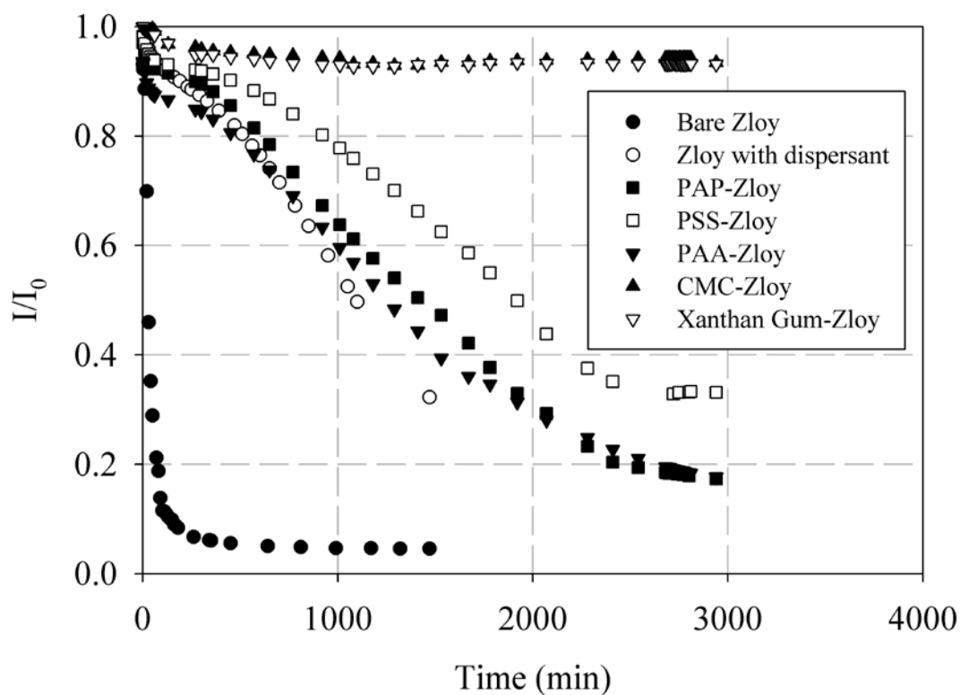
Figure 7.7.5 Sedimentation curves of Z-Loy modified with various macromolecules
