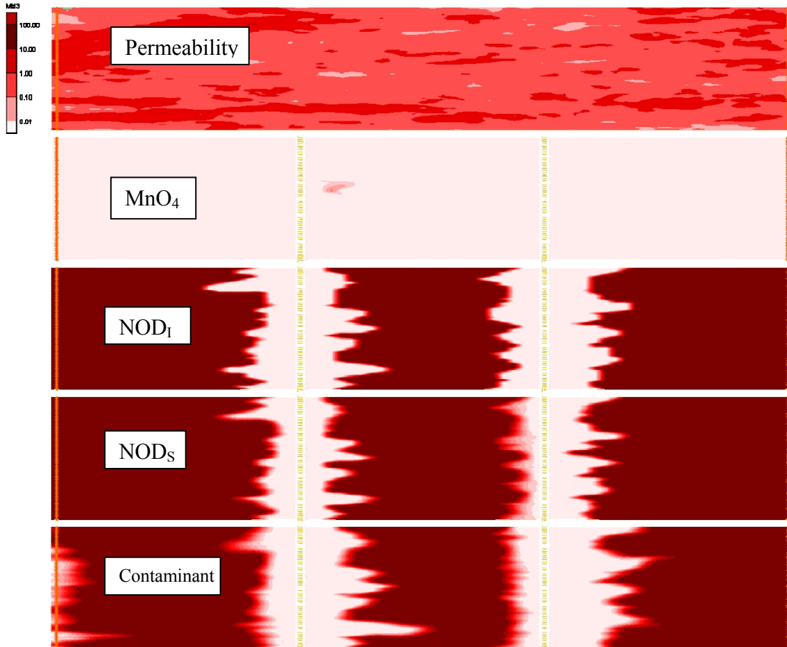
Figure 5.4: Horizontal hydraulic conductivity, MnO_4 , NOD_I , NOD_S and contaminant distribution in last row of aquifer (bottom row of Figure 5.3) at 120 days after injection for moderately heterogeneous aquifer (realization #3) when wells 1-5 are injected with SFV = SFM = 0.25 . Deep red indicates a very high concentration or value, white indicates very low or zero.
