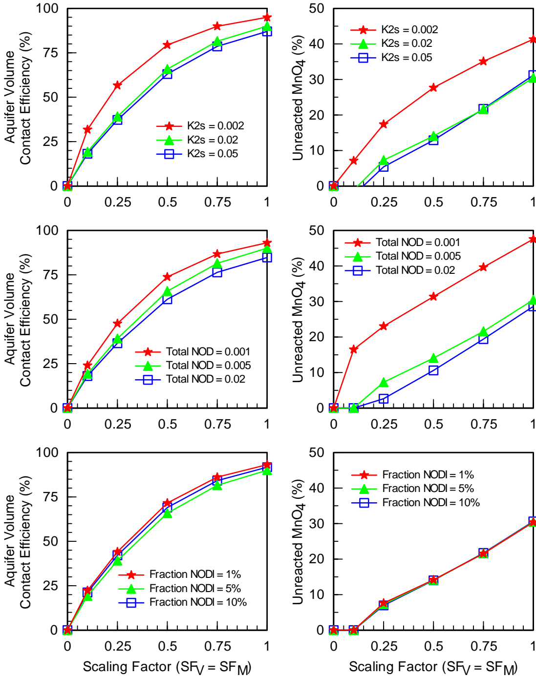
Figure 5.9: Effect of NOD Kinetic Parameters on E_V and U at 180 days for SF_V=SF_M : (a) Slow NOD Reaction Rate ( k_{2s} ); (b) Total NOD; and (c) Fraction NOD_I .
