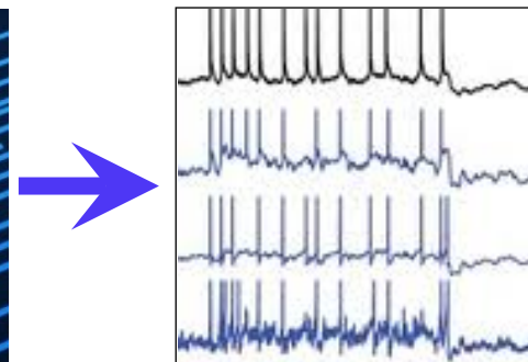
(Neural data)
