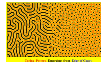
Turing Pattern Emerging from Edge of Chaos
