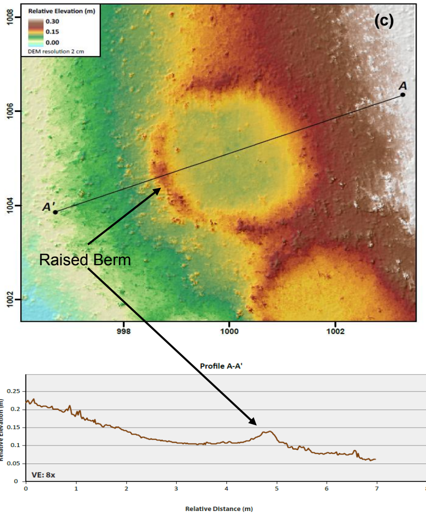
Figure 3.6. Examples of the application of LiDAR in the study of cleared circles at YPG. (a) Leica Geosystems ScanStation™ II; (b) Cyclone visualization snap shot of the LiDAR scan of cleared circles showing well-defined smooth central area (high laser reflectance) and apparent topography associated with the rim; (c) Microtopographic profile across cleared circle along A-A' (McDonald et al., 2011).
