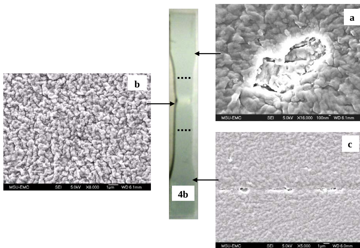
Figure 9 Plastic deformation of spherulites; microvoid formation in spherulites of PP. Images are from a moderately deformed tensile bar exploring the differences between regions. In general, the central region of the sample was more deformed than the outside regions.
