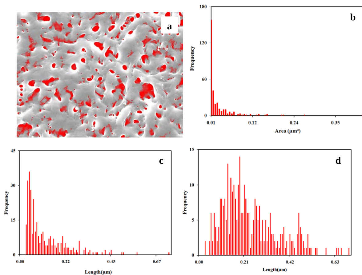
Figure 8 Image with highlighted pores obtained form ImageAnalyzer program (a) frequecy to area graph (b), frequency to diameter graph (c), and frequency to nearest neighbor distance (d)
