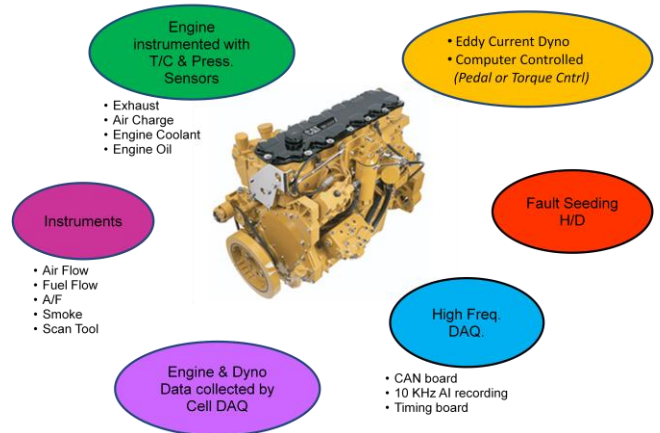
Figure 1. Schematic view of the instrumentation used in the experiments.
