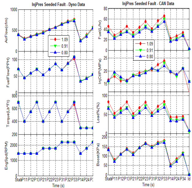
Figure 11. Mean values of engine operating parameters at different speed/torque points as given in Table 3 without the low torque points. The gain change applied to the Control Pressure is indicated in the legend. These tests were carried out with the dyno operating in speed/torque control mode.
