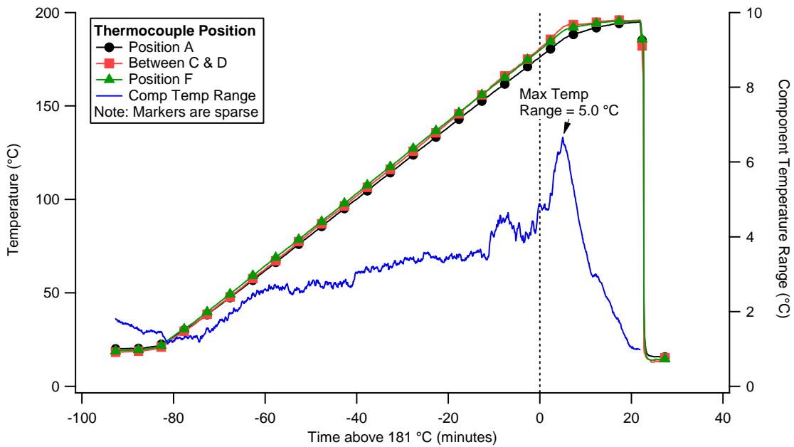
Figure 16: Temperature-time data collected from the thermocouples attached to the component during the retrogression of Component 5. The component temperature range is the difference between the hottest and coldest thermocouples.
