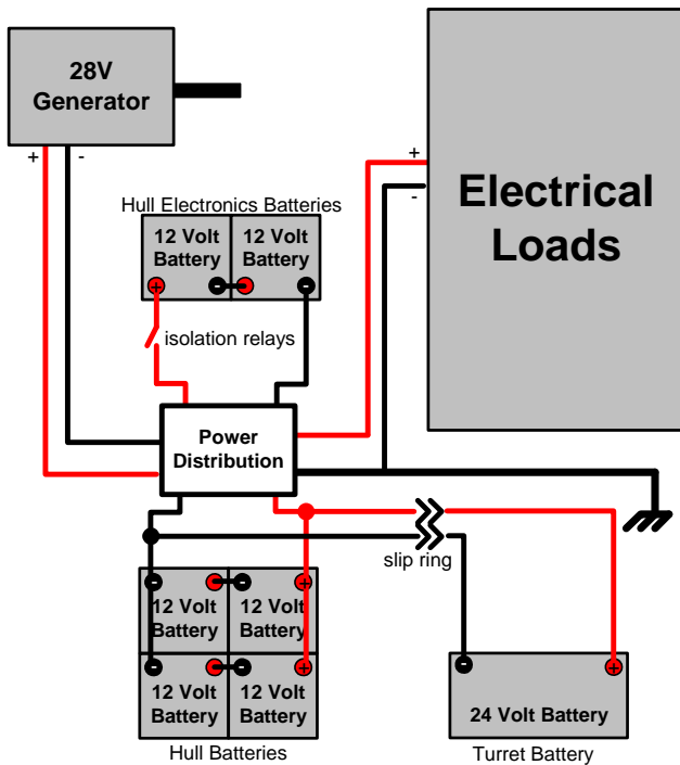
Figure 2: Simplified IFV Electrical Schematic
