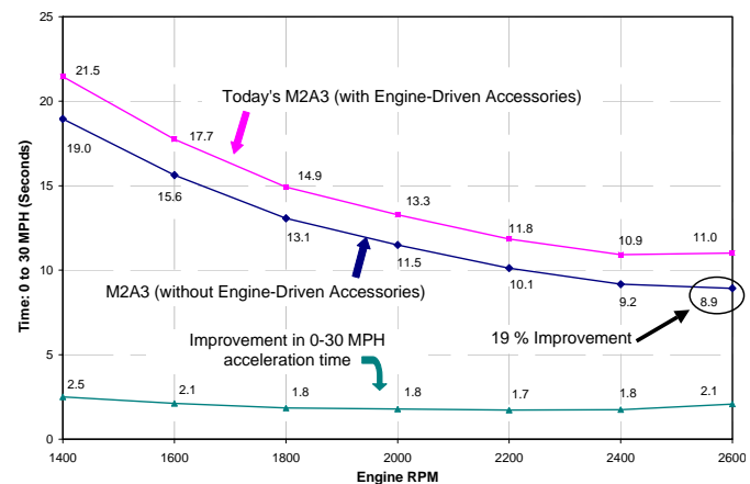
Figure 8: Improvement in 0 - 30 MPH Acceleration
