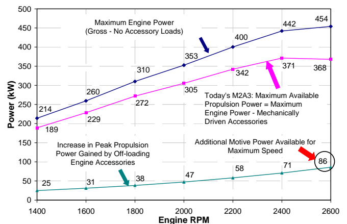
Figure 7: Improvement in Peak Engine Power
