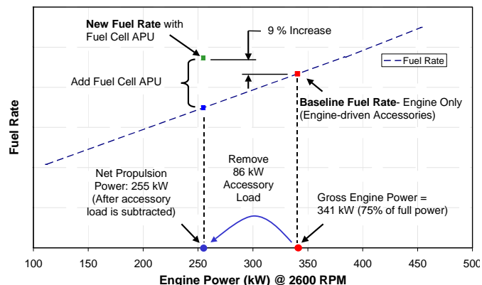
Figure 9 Fuel Economy Impact
