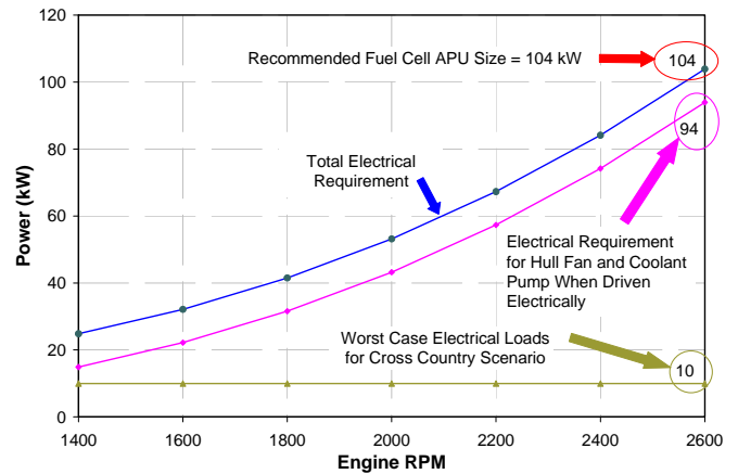
Figure 6 Powering Accessories: Electrical Sizing of APU
