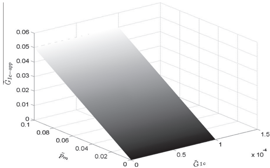
Fig. 12. Apparent fracture toughness as a function of maximum friction force and interlaminar fracture toughness.
