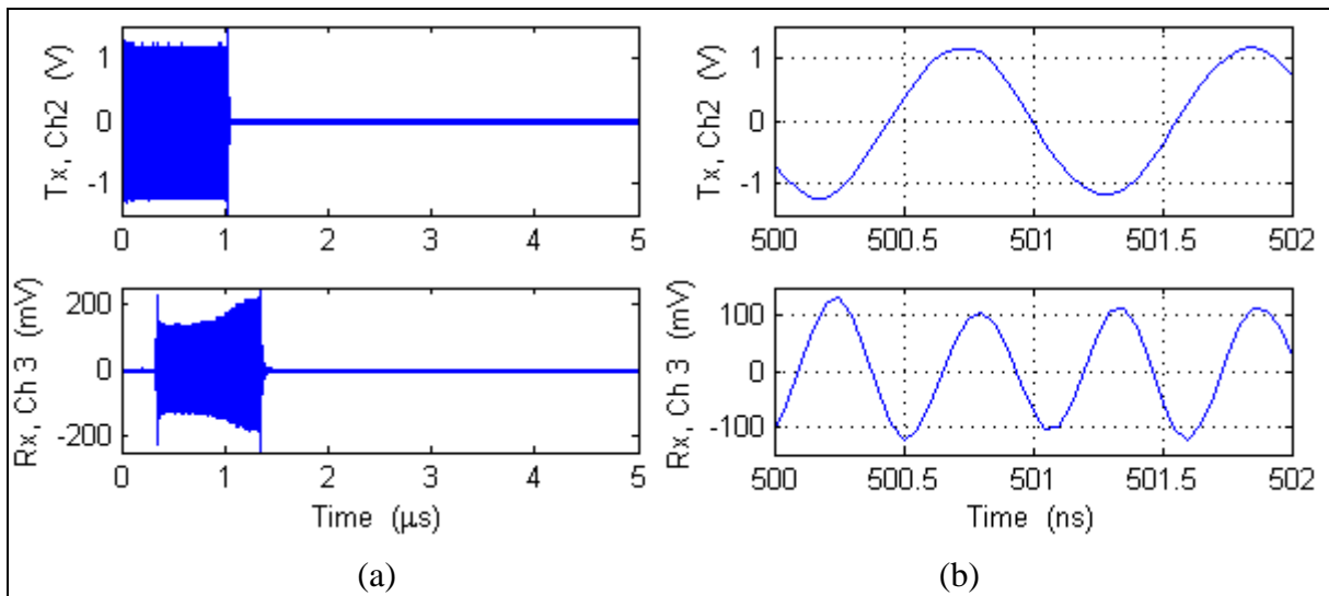
Figure 14. Radar data, RF pulse Tx waveform, linear Rx mode, FRS radio target: f_{pulse} = 900 MHz, P_{env} = 0 dBm, T_{env} = 1 \mu s, D_c = 10\% , (a) raw data, complete time scale and (b) raw data, zoomed-in time scale.
