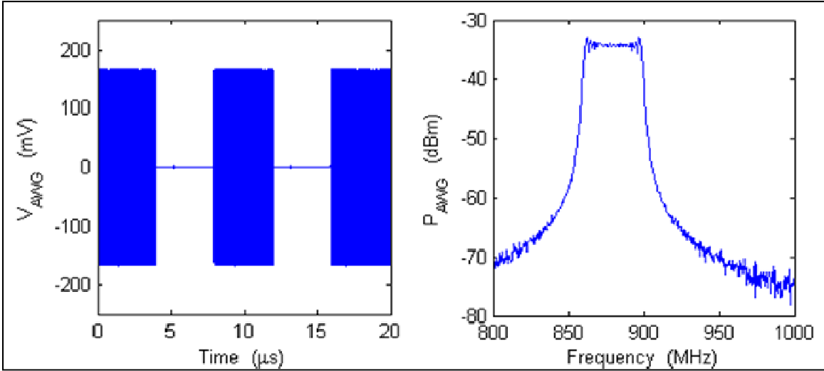
Figure 6. Linear FM chirp pulse output by AWG: f_{\text{start}} = 860 MHz, f_{\text{end}} = 900 MHz, P_{\text{env}} = -3 dBm, T_{\text{env}} = 4 \mu\text{s} , D_c = 50\% .
