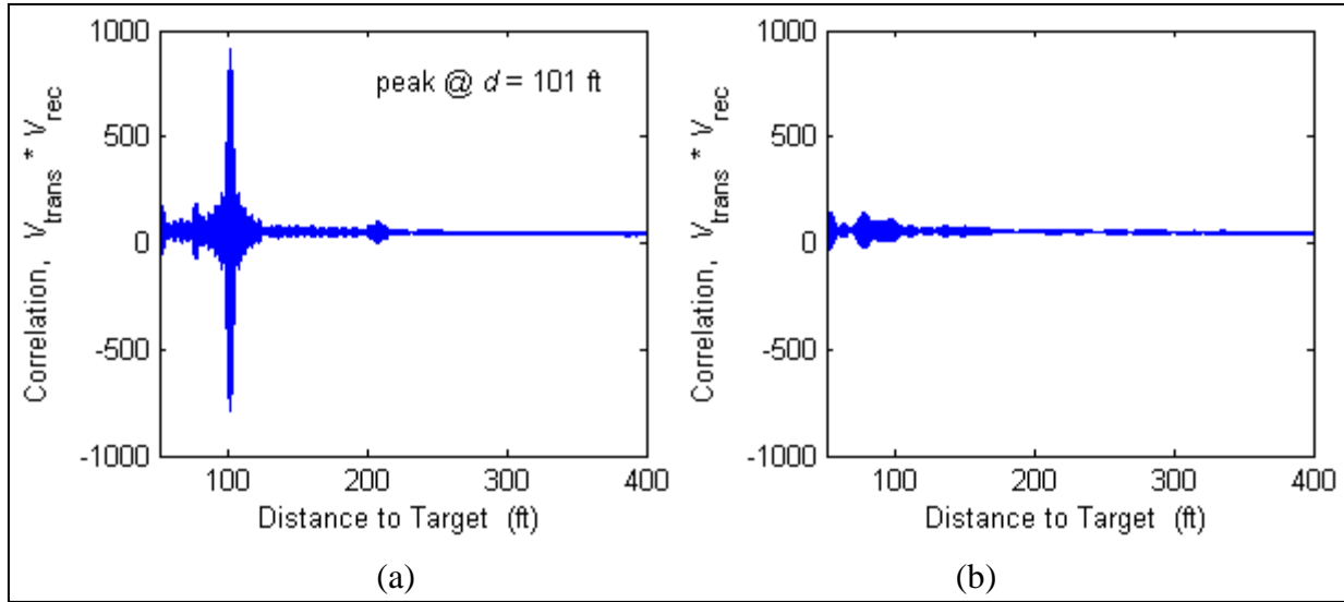
Figure 13. Radar data, chirp Tx waveform, linear Rx mode: f_{start} = 860 MHz, f_{end} = 940 MHz, P_{env} = 0 dBm, T_{env} = 1 \mu s, D_c = 10\% , (a) open-circuit target, (b) matched-load target.
