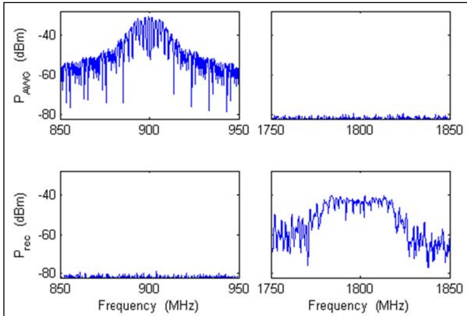
Figure 15. Tx and Rx frequency content, stepped-frequency Tx waveform, nonlinear Rx mode, FRS radio target: f_{start} = 890 MHz, f_{end} = 910 MHz, \Delta f = 1 MHz, P_{env} = 0 dBm, T_{env} = 2 \mu s, D_c = 20\% .
